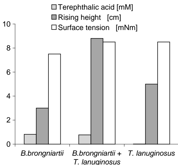
Figure 3. Hydrophilicity of PET samples and concurrent release of terephthalic acid after treatment with enzyme preparations from B. brongniartii ( 0.5 \text{ nKat mL}^{-1} ) and T. lanuginosus ( 5 \text{ nKat mL}^{-1} ) and a combination of both ( 0.5 \text{ nKat mL}^{-1} B. brongniartii and 5.0 \text{ nKat mL}^{-1} T. lanuginosus ). The rising height and surface tension of control samples were 0 cm and 6.2 mNm, respectively.
