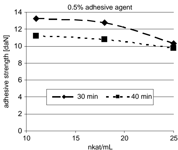
Figure 5. Adhesiveness values for PVC-coated PET material treated at pH 7 for 30 and 40 min with varying activities of the T. lanuginosus enzyme preparation using 0.5% of adhesive agent in the first coating layer
