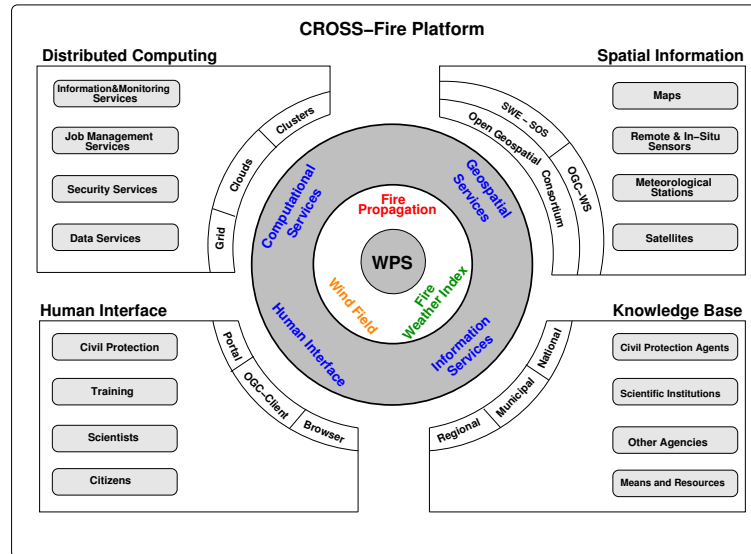
Fig. 1. CROSS-Fire Platform Architecture
