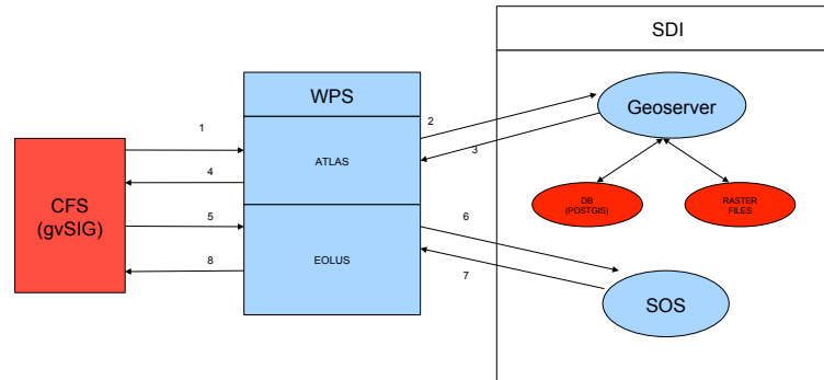
Fig. 3. Phase 1 - Data Requests
