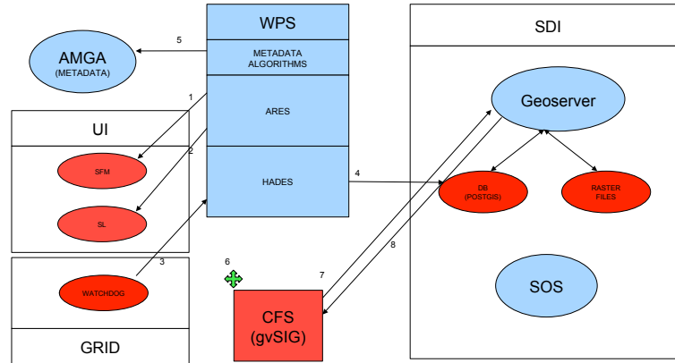
Fig. 5. Phase 3 - Simulation Launching
