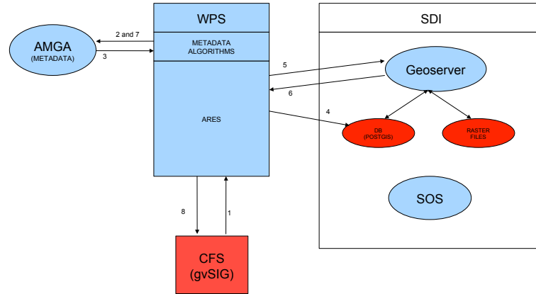
Fig. 4. Phase 2 - Simulation Data Infrastructure
