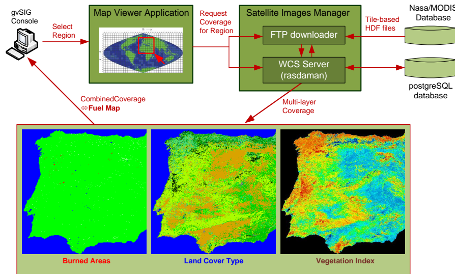
Fig. 6. Illustration of the computation of dynamic fuel map with data from MODIS.
