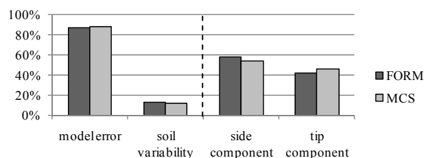
Figure 2: Influence of each uncertainty(%) in pile RBD
