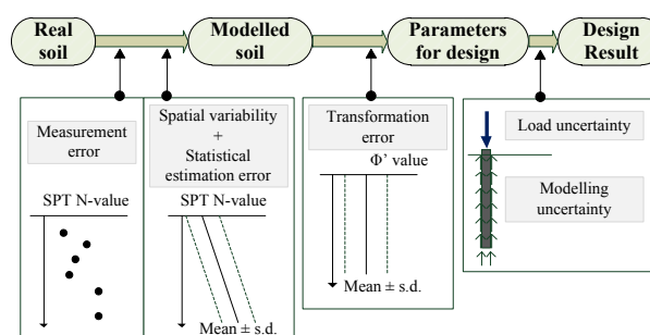
Figure 1: Methodology and uncertainties considered for reliability based design (RBD) of pile foundations
