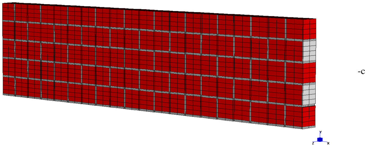
Figure 9: Stretcher bond masonry parapet subject to low velocity impact. –a: FE limit analysis discretization. –b: elastic-plastic 2.5D model discretization (WI2.5D). –c: elastic-plastic 3D model discretization (WI3D). Only \frac{1}{2} of the wall is analyzed for symmetry.
