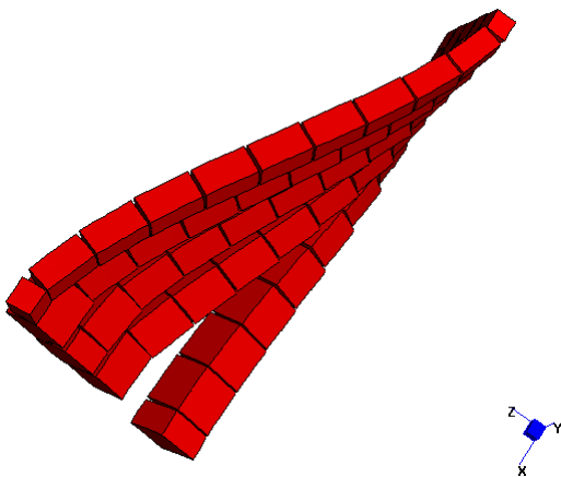
Figure 10: Stretcher bond masonry parapet subject to low velocity impact. Comparison among deformed shapes at t=100 msec –a: Homogenized limit analysis approach. –b: heterogeneous 2.5D elastic-plastic FE approach. –c: heterogeneous 3D elastic-plastic FE approach. Only \frac{1}{2} of the wall is analyzed due to symmetry.
