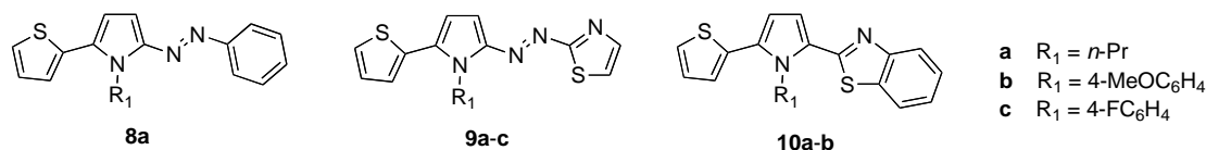
Figure 1. Structure of thienylpyrrole derivatives 8a , 9a-c and 10a-b . 8d,8g
