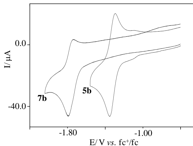
Figure 2. Cyclic voltammograms for the first reduction step of compound 5b and 7b ( 1.0 \times 10^{-3} \text{ mol dm}^{-3} ) in DMF, 0.1 \text{ mol dm}^{-3} [\text{NBu}_4][\text{BF}_4] at a vitreous carbon electrode, between -0.6 \text{ V} and -2.10 \text{ V vs. fc}^+/\text{fc} , scan rate 0.1 \text{ V s}^{-1} .
