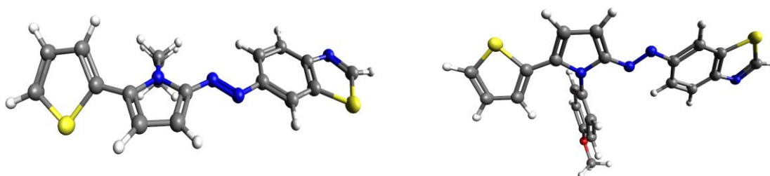
Figure 5. Ground-state molecular structures for azo dyes 7a (left) and 7b (right) optimized using B3LYP/6-31+G(d,p).
