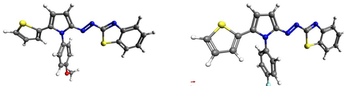
Figure 4. Ground-state molecular structures for azo dyes 5b (left) and 5c (right) optimized using B3LYP/6-31+G(d,p).
