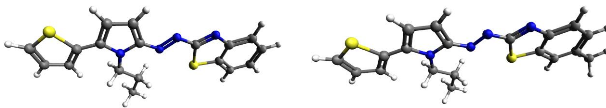
Figure 3. Ground-state molecular structures for azo dyes 5a (left) and 6a (right) optimized using B3LYP/6-31+G(d,p).
