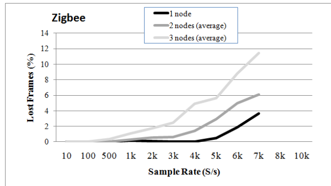
Fig. 12. Lost frames, low-power module using Zigbee, variable number of nodes
