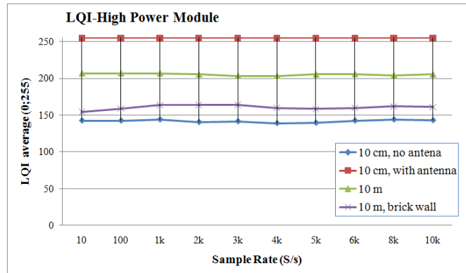
Fig. 6. Link quality indicator throughout the experiment, high power module
