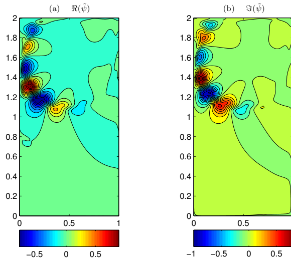
Fig. 3. Eigenfunctions of the streamfunction for lid-driven cavity at a critical Reynolds number of Re = 8026.7 and aspect ratio A = 1 .
