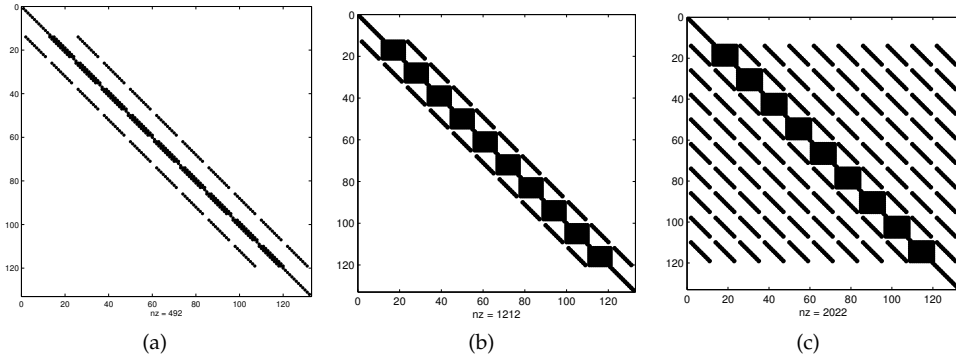
Fig. 1. Sparsity patterns for model problem with (a) second order finite-differences in both x and y with N = 10, M = 11 , (b) second-order finite-difference in x and chebychev collocation in y with N = 10, M = 11 , (c) chebychev collocation in both x and y with N = 10, M = 11 .
