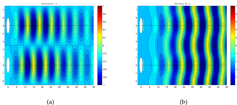
Fig. 5. Perturbation eigenfunctions the flow past a circular cylinder for a gap width W = 5 with (a) anti-phase oscillatory mode, (b) in phase oscillatory mode.
