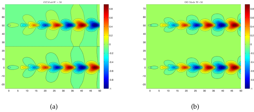
Fig. 6. Perturbation eigenfunctions the flow past a circular cylinder for a gap width W = 50 with (a) anti-phase oscillatory mode, (b) in phase oscillatory mode.
