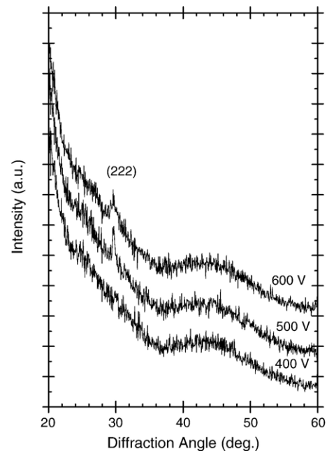
Fig. 1. XRD spectra of the ITO films deposited at different screen voltage.
