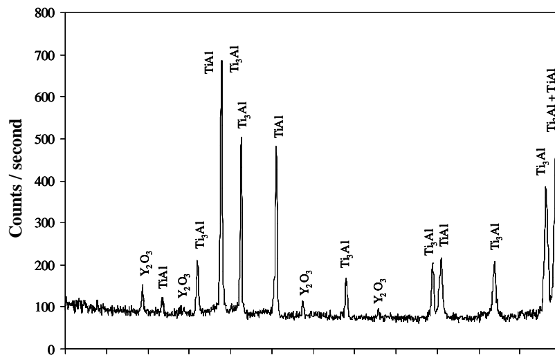
Figure 3. X-Ray Diffraction spectrum of the sample obtained in Y_2O_3 partially stabilized ZrO_2 crucibles with inside Y_2O_3 layer, showing the co-existence of Ti_3Al , TiAl and Y_2O_3 .
