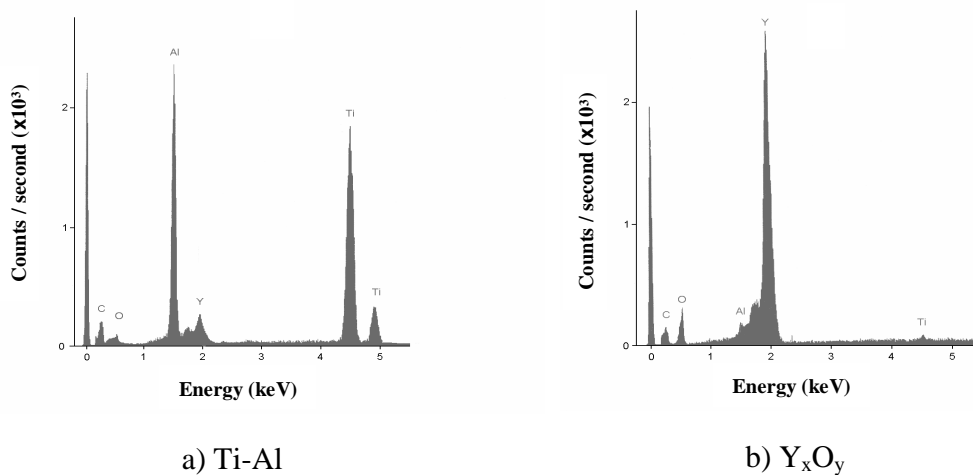
Figure 9. EDS spectrum of the constituents present on the microstructure shown on figure 8 b).
