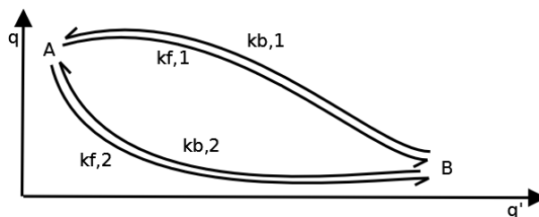
Figure 1: Diagram of a system described by two reaction coordinates q and q' with two stable states A and B connected by two distinct processes 1 and 2. k_{f,1} and k_{f,2} are the forward rate constants for either process; k_{b,1} and k_{b,2} the backward rates.
