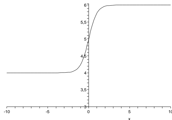
Figure 1: Exact traveling wave profile solution for the gas density ( \rho versus space).
