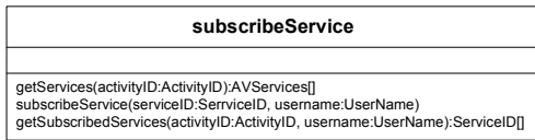
Figure 7. Attributes and methods for the subscribeService class
