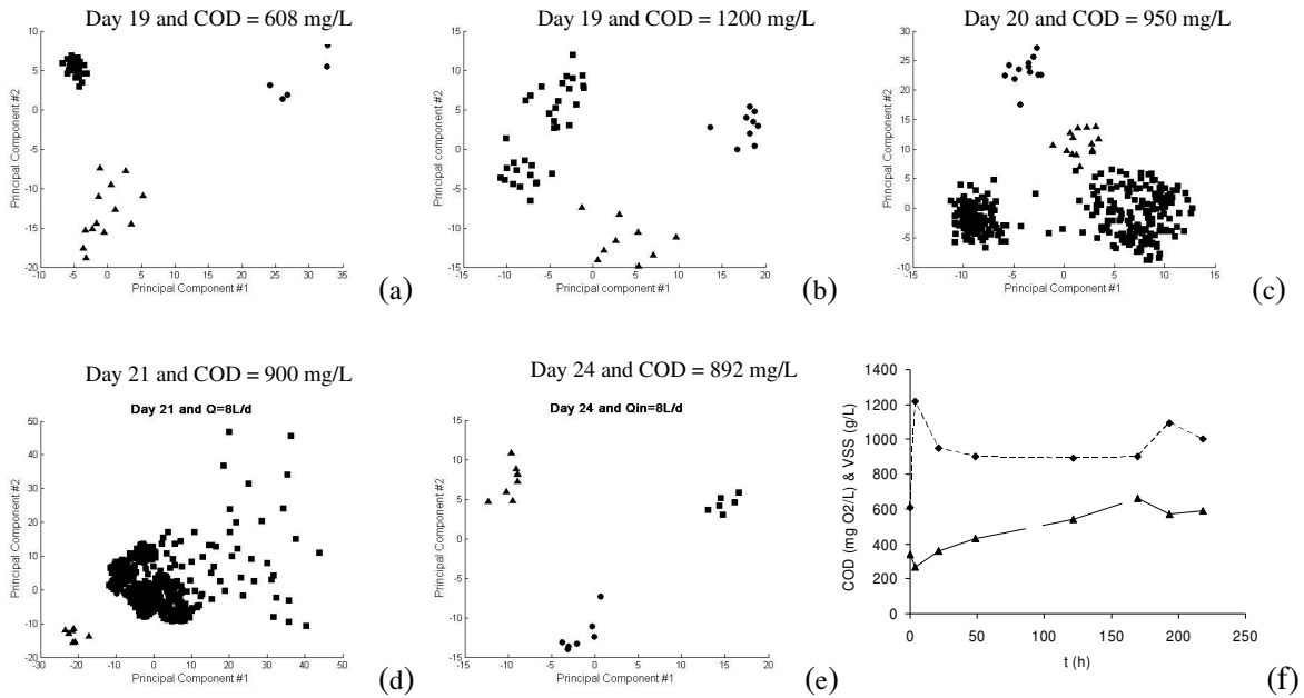
Figure 6. Evolution of the state of an aerobic biological reactor monitored through the analysis of score plots including the three monitored points of the reactor: Feed (●), Reactor (■) and Settler (▲). Figure (f) represents the evolution of the COD in the feed and the VSS in the reactor.
