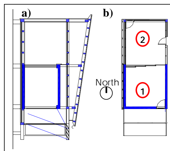
Fig. 2. Plants of the STC; a) lateral; b) top.
