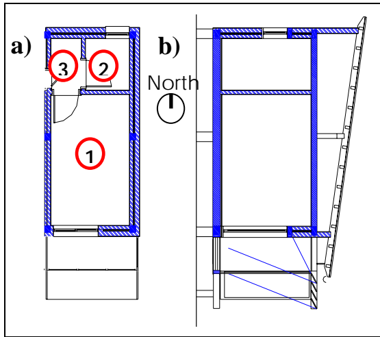
Fig. 3. Plants of the STC; a) top; b) lateral.
