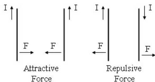
Figure 8. Forces between two parallel conductors
