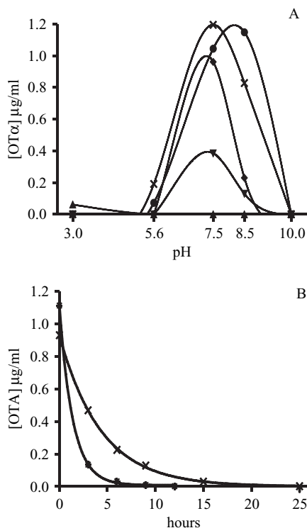
Figure 5: (A) Activity at different pH and 37°C of the enzymes, expressed in ochratoxin \alpha concentration. (- \blacktriangle -, Prolve PAC; - \blacktriangledown -, pancreatin; - \blacklozenge -, Protease A; - \bullet -, Carboxypeptidase A and - \times -, Ancex); (B) comparison between ochratoxin A hydrolysis activity of Ancex at pH 7.5 and 37°C (- \times -) and Ancex at pH 7.5 and 50°C (- \ast -).
