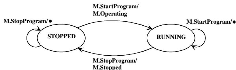
Figure 3: State diagram for MachineTool module
