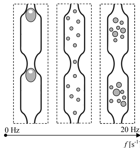
Figure 2. Identified bubbles behaviour with increasing f .
