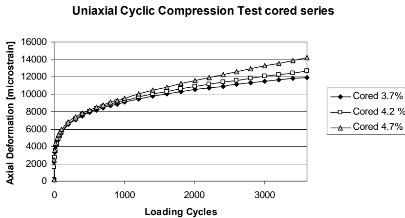
Figure 6. Relation between the Bitumen content and the deformation rate in the Uniaxial Cyclic Compression Test
