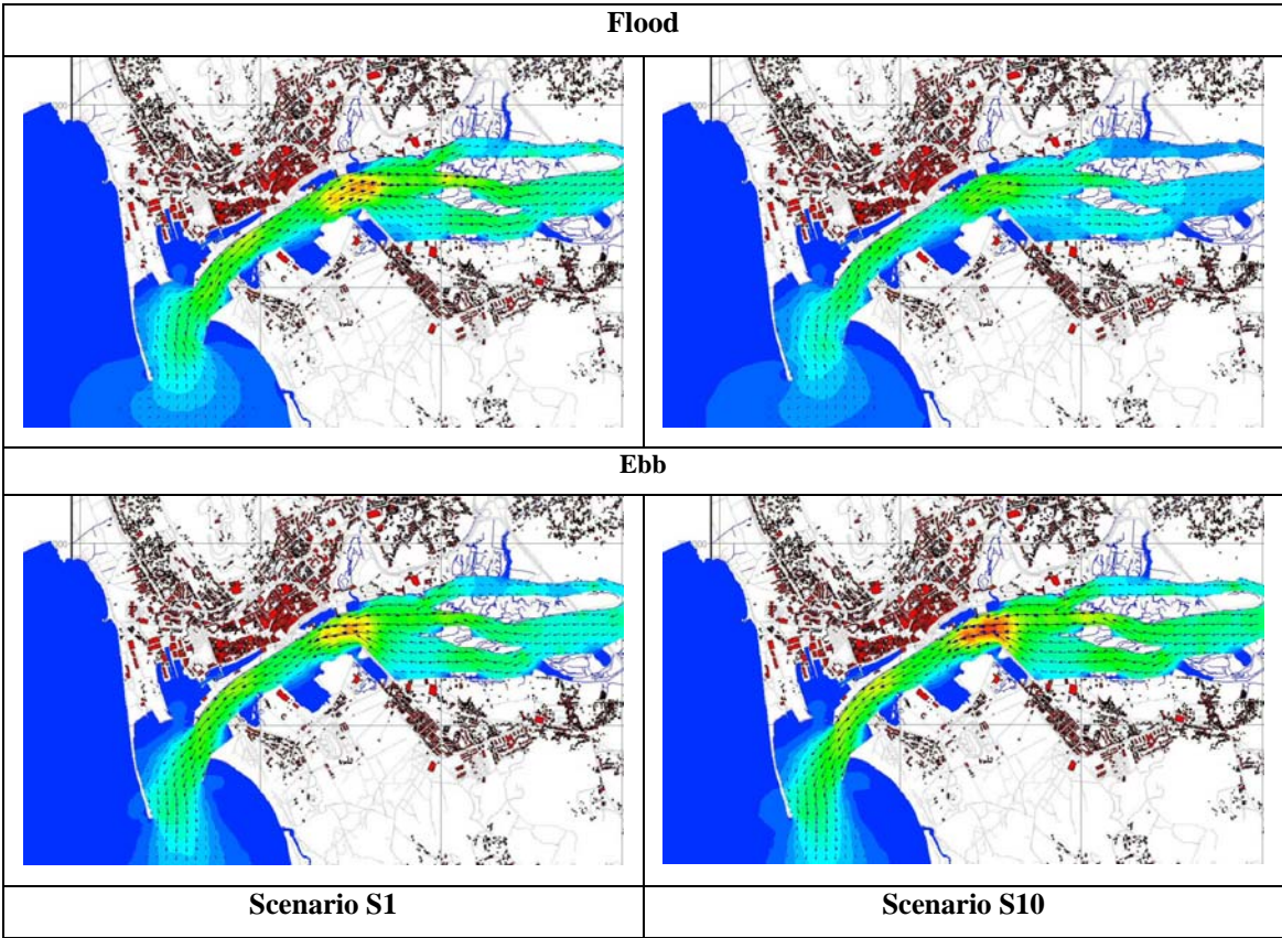
Fig. 4 Hydrodynamic model: current velocities for the harbour zone during ebb and flood for scenarios S1 and S10.
