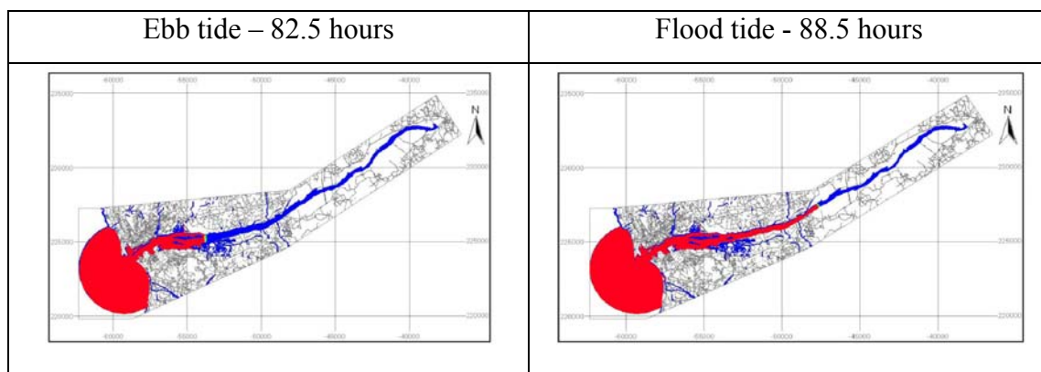
Fig. 6 Mass transport model: intrusion extent during ebb and flood under conditions of scenario S1
