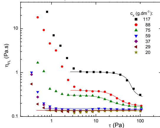
Figure 3. Viscosity curves as a function of shear stress, \tau , for different biomass concentrations, c_X . The lines represent the fittings using the Cross model. All measurements were performed at 30 \text{ }^\circ\text{C} .
