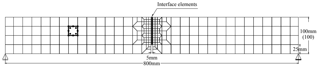
Fig. 4 - Finite element mesh adopted in the numerical simulation
