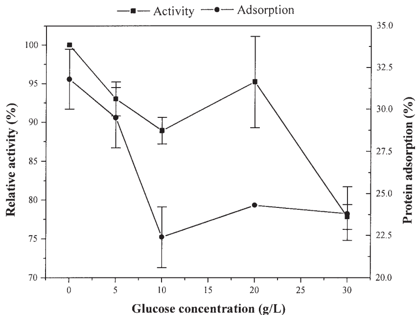
Fig. 2. Effect of glucose concentration on cellulase (TC) activity and adsorption (50°C, pH 5.0, 3.8 mg protein/g fabric). The values in the figure represent the mean of two independent experiments and error bars the standard deviation.
