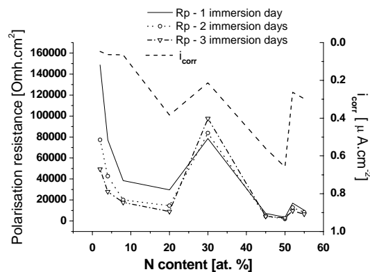
Fig. 6. Influence of the nitrogen amount and immersion time on polarisation resistance of the samples. For comparison, the evolution of i_{\text{corr}} with the nitrogen content is also plotted in the graph.
