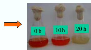
Figure 2: Aspect of the flasks after 0, 10 and 24 hours of growth.
