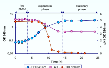
Figure 1: Typical growth and decolourisation curve of UM41 on NDM in the presence of dye II.
