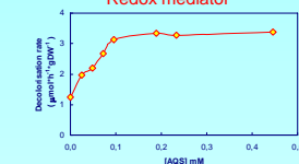
Figure 8: Effect of the redox mediator on the decolourisation rate.
