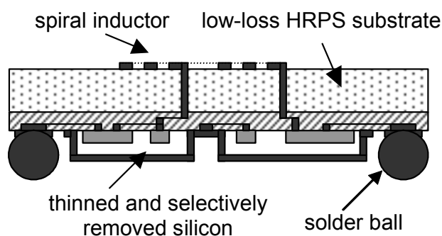
Fig. 1: Schematic view of the proposed wafer-level packaging concept based on a low-loss high-resistivity polycrystalline silicon substrate enabling vertical spacing of RF passive components (e.g. large spiral inductors).
