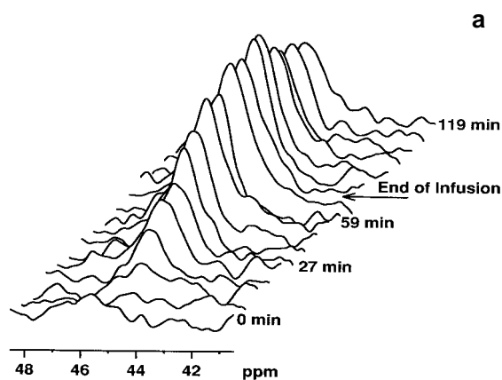
Figure 4 (a) Stack plot of the ^{27}\text{Al} NMR spectra of the in vivo experiment with Al(NOTA) in a rat. For one spectrum 2000 scans were accumulated. Prior to Fourier transformation the spectral data were treated with a 40 Hz Gauss filter. The linewidth was (unfiltered) 95 Hz. The in vivo signal appears circa 4 ppm lower (45 ppm) than in vitro . As marked with an arrow the infusion was stopped and the signal intensity decreased. (b) Time course of the signal intensity (integrated area) of the spectra. The linear decrease of the signal intensity demonstrates a constant clearance rate.
