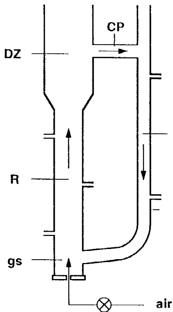
Figure 1. Schematic diagram of the experimental bioreactor; R (riser); D (downcomer); DZ (deceleration zone); gs (gas sparger); CP (connection pipe).
