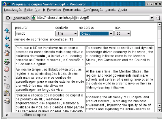
Figure 2: Querying the extracted corpus with a CGI
