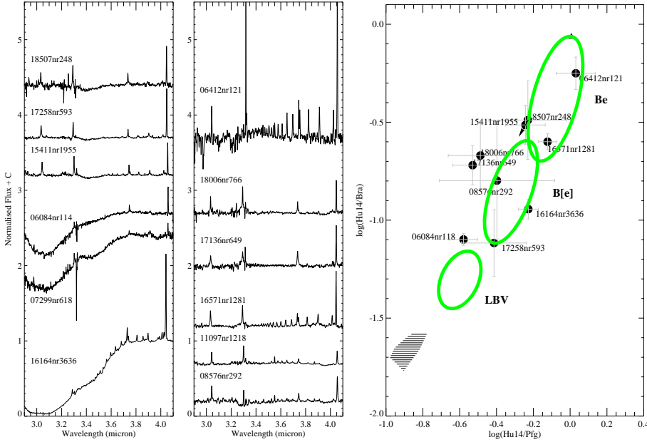
Figure 1. left 2 pannels : L-band spectra taken with ISAAC at the VLT of 12 massive YSOs. The broad absorption are molecular solid-state transition features caused by material in the diffuse ISM or molecular clouds. These absorption features can be used to derive an accurate line-of-sight extinction value. The emission lines are mainly hydrogen emission lines. The lines needed to construct the diagnostic diagram are Br \alpha (4.05 \mu m), Pf \gamma (3.754 \mu m) and Hu14 (4.02 \mu m). right : The L-band diagramme as described in the text. The gray circles represent the loci of the massive stars with known circumstellar geometry for which Lenorzer et al. (2002) constructed the diagramme: LBVs, B[e] and Be stars. Overplotted are the massive YSOs.
