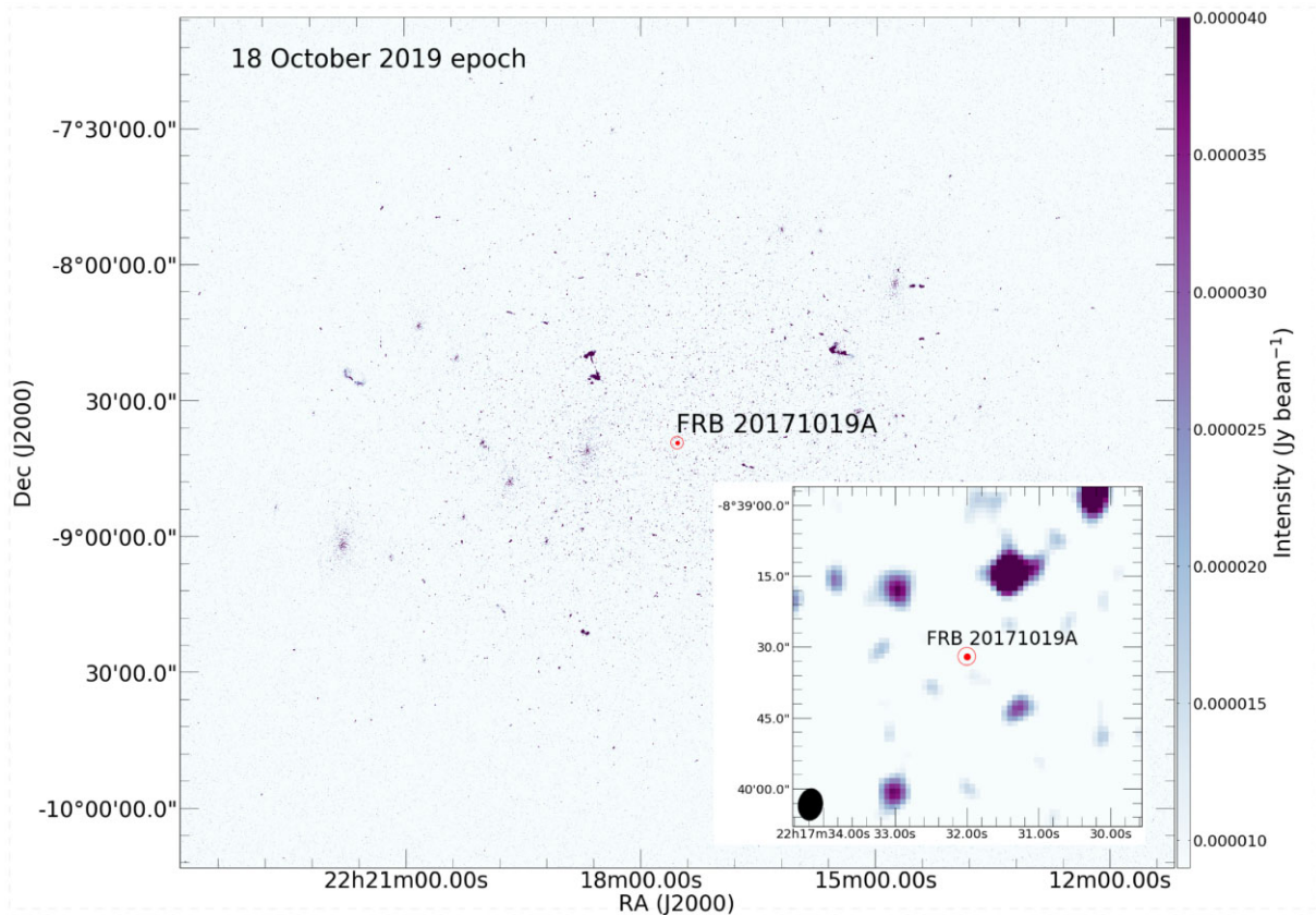
Figure 7. FRB 20171019A MeerKAT image and a zoom-in (insert) around the position of the FRB. The black ellipse on the bottom left corner of the insert represent the beam size of MeerKAT.
