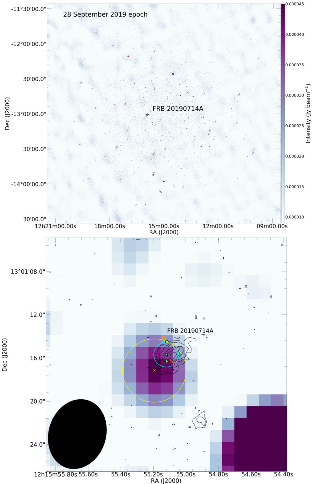
Figure 3. Top: MeerKAT image of FRB 20190714A from 2019 September 28 (bottom) and the zoom-in image centred around the position of FRB 20190714A. Contours (levels: 300, 500, 900, 1200, 1600 counts) represent the PanSTARRS i -band optical counterpart of the spiral galaxy coincident in position with the persistent radio emission. The black ellipse in the lower left corner represents the MeerKAT beam size. The light green star and cyan circle represent the position of the FRB and the 2\sigma total uncertainty in the position as determined by the ASKAP detection (Day et al. 2021). The two light green filled circles represent the peak of the two compact persistent emission (north and south indicated with orange N and S) detected with e-MERLIN. The yellow cross and yellow circle represent the peak of the MeerKAT emission and the 2\sigma uncertainty on the position, respectively.
