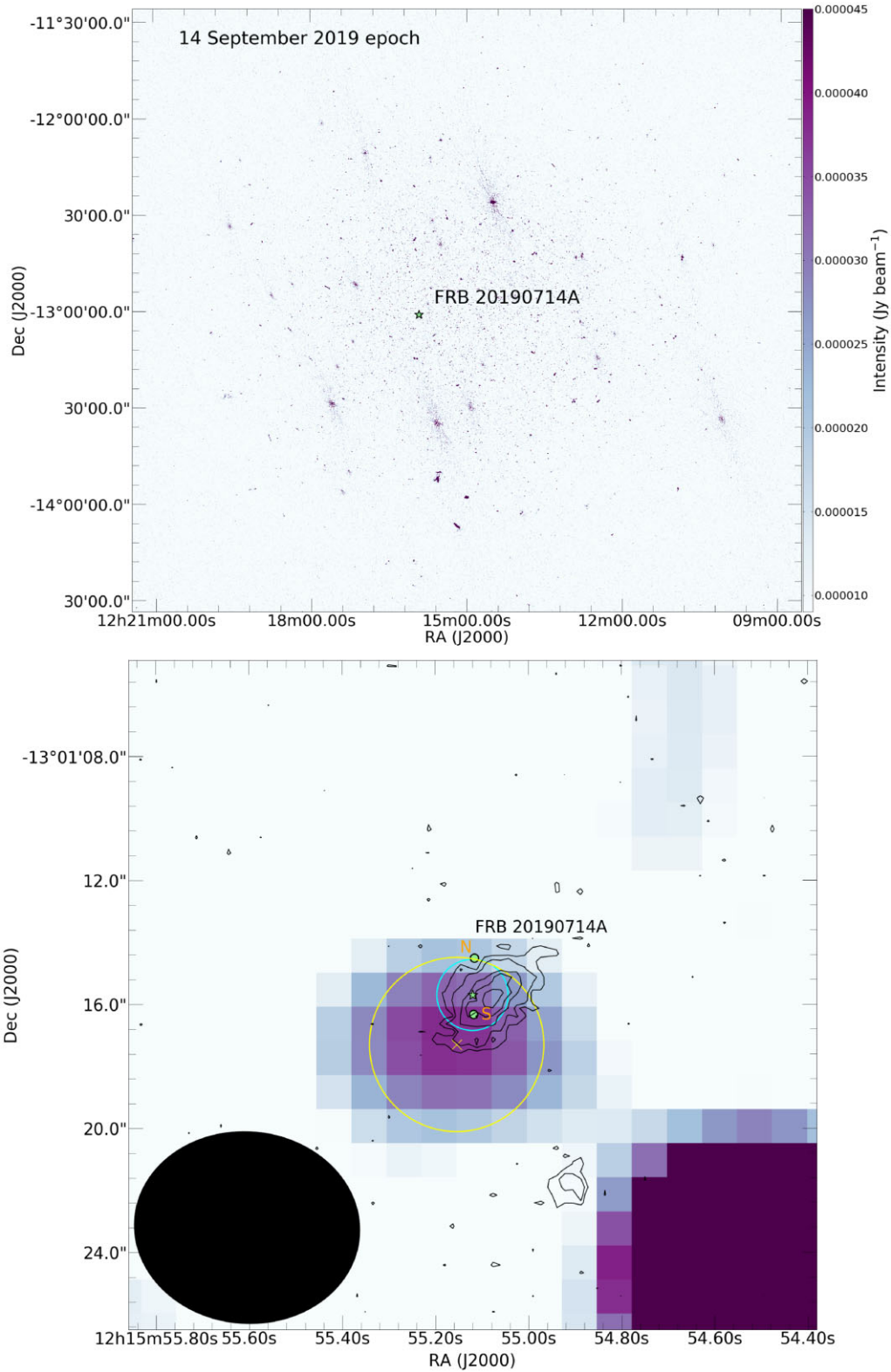
Figure 2. Top: MeerKAT image of FRB 20190714A from 2019 September 14 (bottom) and the zoom-in image centered around the position of FRB 20190714A. Contours (levels: 300, 500, 900, 1200, 1600 counts) represent the PanSTARRS i -band optical counterpart of the spiral galaxy coincident in position with the persistent radio emission. The black ellipse in the lower left corner represents the MeerKAT beam size. The light green star and cyan circle represent the position of the FRB and the 2\sigma total uncertainty in the position as determined by the ASKAP detection (Day et al. 2021). The two light green filled circles represent the peak of the two compact persistent emission (north and south indicated with orange N and S) detected with e-MERLIN. The yellow cross and yellow circle represent the peak of the MeerKAT emission and the 2\sigma uncertainty on the position, respectively.
