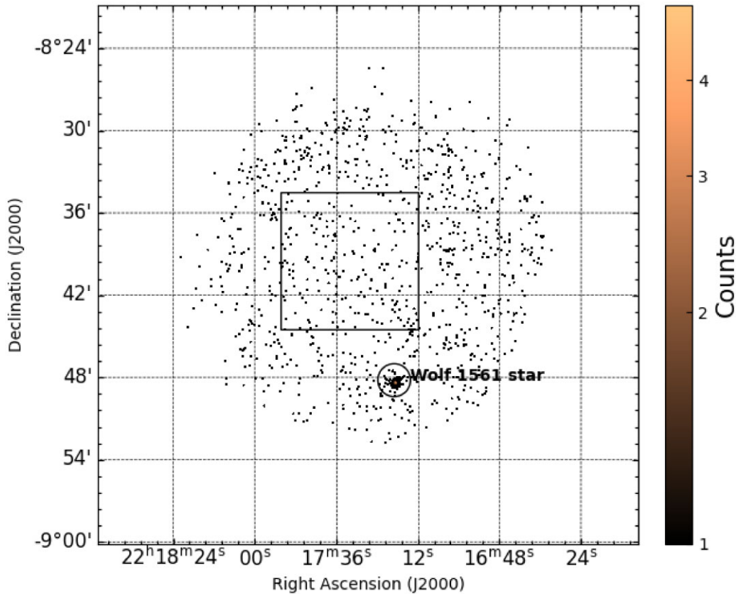
Figure 5. XRT summed image of FRB 20171019A region taken during the MWL observation campaign in 2019 September–October. The position of the Wolf 1561 star is indicated with the black open circle and labelled. The black box indicates FRB 20171019A 90 per cent localization region as reported in Kumar et al. (2019).
