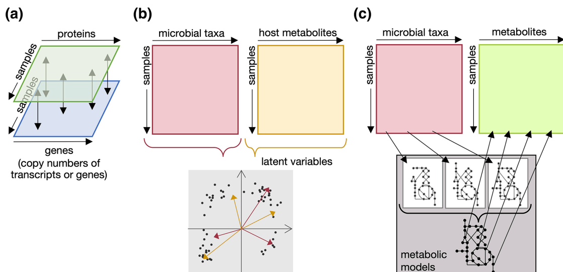
Figure 2. Schematic representation of integration strategies. Each meta-omics data set is visualized as a matrix of samples \times analytes. In all examples, the samples that are measured at the two meta-omics levels are representative of the same systems. (a) Due to sequence identity, the analytes (e.g., proteins and genes) can be directly related across the meta-omics levels; (b) the relationship between the analytes in the two data sets is unknown and data fusion methods are employed to reveal common patterns within the samples (black dots) together with the most important analytes (arrows); (c) for well-described systems, links between the analytes in the two data sets are established based on existing knowledge, e.g., genome scale metabolic models. Metabolic models of each species (white boxes) are combined into common compartment models of the whole community and their host (grey box), of which the metabolites are obtained. Approaches to extending metabolic models to community level are still in their infancy.
