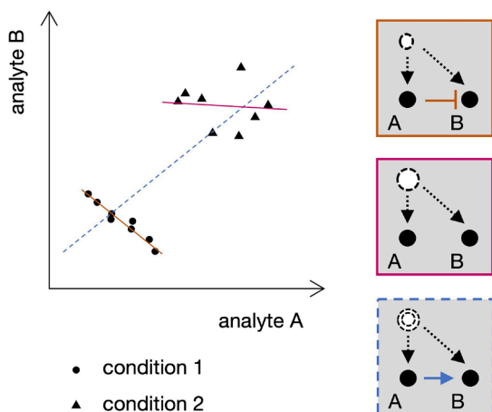
Figure 4. The interpretation of correlations between analytes depends fully on the relationship between the samples. Here, analytes A and B are limited by a third (white circle in the boxes, e.g. a precursor or nutrient source) which has one fixed level under condition 1 and another under condition 2. The correlation between analytes A and B over all samples of both conditions simultaneously is positive (blue box) and could suggest positive feedback from A to B, while focusing on specific conditions, negative correlation by inhibition (orange) or no correlation (red) should be concluded.
