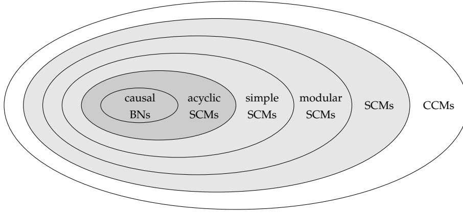
Figure 2.7: Overview of causal graphical models. The “gray” and “dark gray” areas contain all the causal graphical models that can be modeled by an SCM and an acyclic SCM, respectively.
