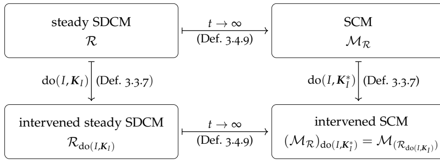
Figure 3.1: This diagram shows that, under certain convergence assumptions, equilibration (left-to-right in the diagram) commutes with intervention (top-to-bottom in the diagram). The precise statement is made explicit in Theorem 3.4.18.
