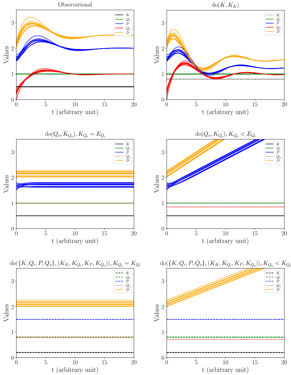
Figure 3.10: Simulation of solutions of the SDCM of the bathtub model of Example 3.4.20 and 3.4.25 under different steady perfect interventions.
