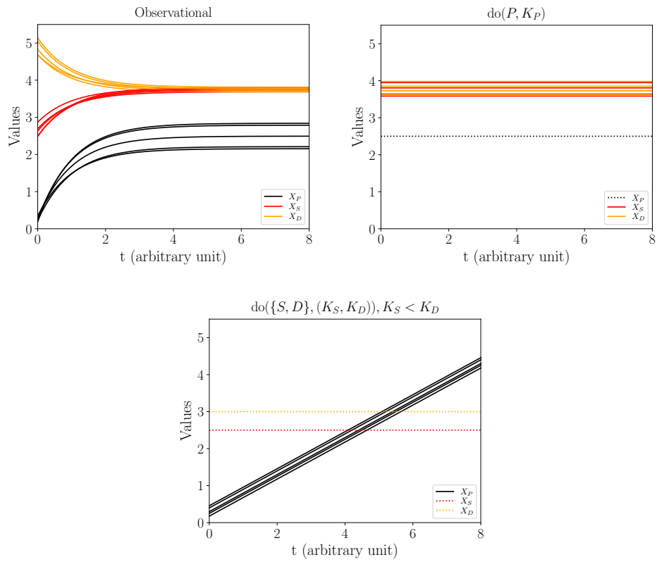
Figure 3.9: Simulation of solutions of the SDCM of the price, supply and demand model of Example 3.4.13 under different steady perfect interventions.
