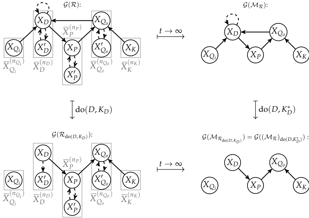
Figure 3.7: Graphs of the bathtub model: original model \mathcal{R} of Example 3.3.30 (top left), the equilibrated model \mathcal{M}_{\mathcal{R}} (top right), the intervened model \mathcal{R}_{\text{do}(D, K_D)} (bottom left), and the intervened and equilibrated model \mathcal{M}_{\mathcal{R}_{\text{do}(D, K_D)}} (bottom right) of Example 3.4.19.
