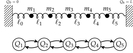
Figure 2.8: Damped coupled harmonic oscillator (top) and the graph of the SCM \mathcal{M} that describes the positions of the masses at equilibrium (bottom) of Example 2.D.1 for d = 5 .
