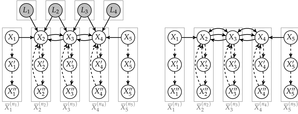
Figure 3.5: Augmented graph (left) and graph (right) of the intervened damped coupled harmonic oscillator model \mathcal{R}_{\text{do}(\{1,5\},(0,L))} of Example 3.3.8 for d = 5 .
