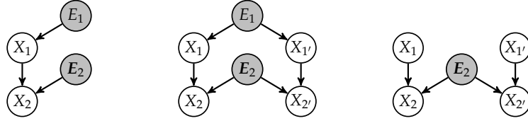
Figure 2.11: The augmented graph of the SCM \mathcal{M}_\rho (left), its twin SCM \mathcal{M}_\rho^{\text{twin}} (center) and the intervened twin SCM (\mathcal{M}_\rho^{\text{twin}})_{\text{do}(\{1',1\},(1,0))} (right) of Example 2.D.7.
