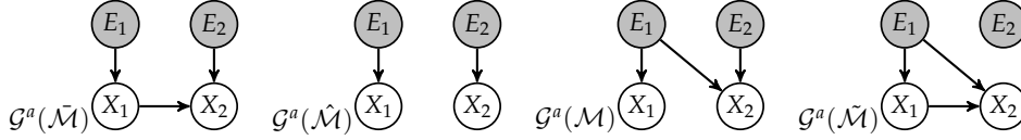
Figure 2.12: The augmented graphs of SCMs \tilde{\mathcal{M}} , \hat{\mathcal{M}} , \mathcal{M} , and \tilde{\mathcal{M}} that appear in Examples 2.4.4, 2.D.10, and 2.D.13.
