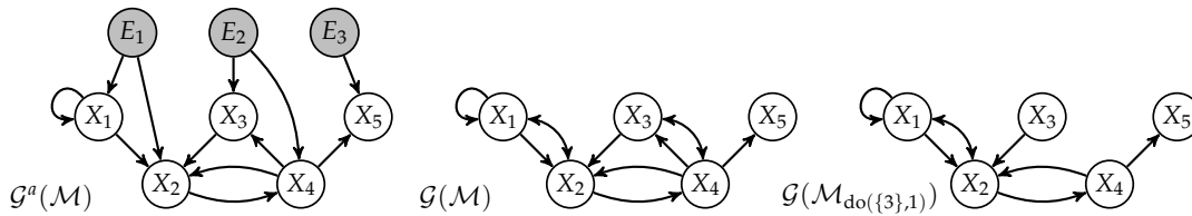
Figure 2.2: The augmented graph (left) and the graph (center) of the SCM \mathcal{M} of Example 2.2.8 and the graph of the intervened SCM \mathcal{M}_{\text{do}(\{3\},1)} of Example 2.2.16 (right).
