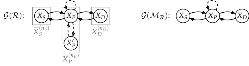
Figure 3.6: Graphs of the price, supply and demand model \mathcal{R} (left) of Example 3.3.15 and the corresponding equilibrated model \mathcal{M}_R (right) of Example 3.4.17.
