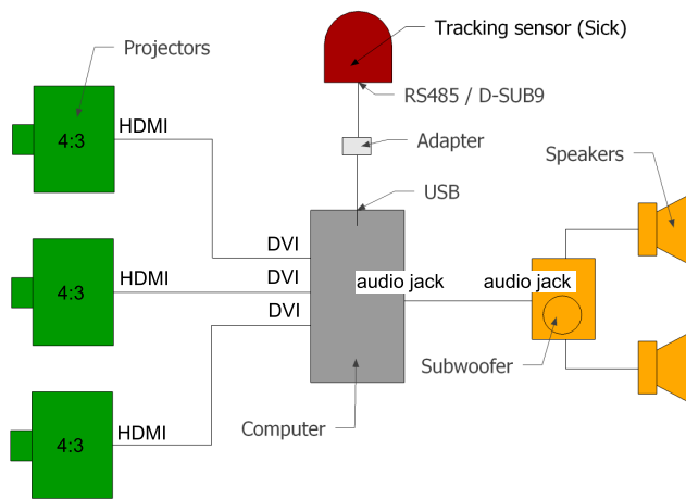
Figure 2: Equipment schematic for Horizons by Geert Mul (artwork creation 2008, version 2013)
