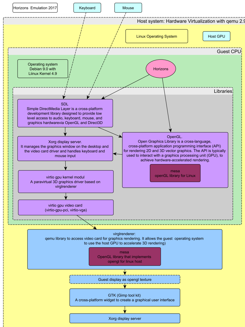
Figure 4: Virtualization of Horizons by migrating it from Debian 7 to Debian 9 with qemu
