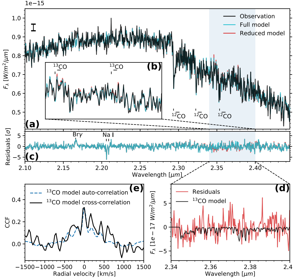
Figure 1 | Observed SINFONI spectrum of exoplanet TYC 8998 b and cross-correlation signal of ^{13}\text{CO} . Panel (a): The observed spectrum is shown in black, the best-fit model including all carbon isotopes in cyan, and the best-fit reduced model, without ^{13}\text{CO} , is shown in red. The typical uncertainty per pixel in the observed spectrum is denoted by the error bar ( 1\sigma ) on the upper left. Sub-panel (b) shows a zoom-in over the 2.34 - 2.40 \mu\text{m} spectral region, centered on the ^{13}\text{CO} bandhead. Specific opacity from ^{13}\text{CO} is located where the reduced model without ^{13}\text{CO} (in red) is higher than the observed spectrum. Panel (c) shows the residuals (spectrum minus best-fit models, with the residuals of the reduced model in red) revealing the Brackett \gamma emission feature at 2.166 \mu\text{m} , and Na I absorption lines. Panel (d): Observational residuals in red are compared with the ^{13}\text{CO} absorption model in black (the difference between the best-fit full model minus the same model with the ^{13}\text{CO} opacity removed), revealing the similarity between the observations and models. Panel (e): Cross-correlation functions (CCF) between observational residuals and the ^{13}\text{CO} model, as shown in black. The dashed line shows the auto-correlation of the ^{13}\text{CO} model, scaled to the peak of the CCF.
