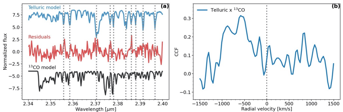
Extended Data Figure 5 | Impact of telluric absorption lines and cross-correlation signal of ^{13}\text{CO} at the extended wavelength region. Panel (a): Comparison of the telluric transmission model with residuals. Some noise is attributed to imperfect telluric correction as noted by dotted gray lines. Panel (b): Cross-correlation function between the telluric model and the ^{13}\text{CO} model, showing no correlation between them.
