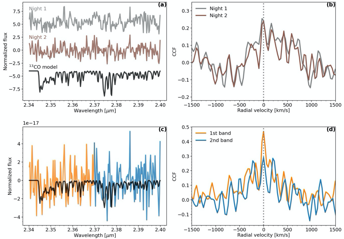
Extended Data Figure 4 | Cross-correlation signal of ^{13}\text{CO} from individual nights and bandheads. Panel (a): observational residuals of two nights separately. Panel (b): cross-correlation signal from individual nights. Panel (c): filtered observational residuals of two ^{13}\text{CO} bandheads separately. Panel (d): cross-correlation signal from individual bandheads.
