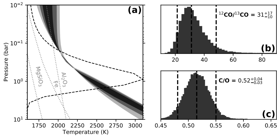
Figure 2 | Spectral retrieval results. (a) The retrieved temperature-pressure profile. The shaded regions with decreasing grey scale show 1\sigma , 2\sigma , and 3\sigma temperature uncertainty envelopes respectively. The gray dotted lines represent the condensation curves of three potential cloud species. The black dashed line shows the flux average of the emission contribution function. (b) Posterior distribution of CO isotopologue abundance ratio ^{12}\text{CO}/^{13}\text{CO} . The vertical dashed lines denote the 5%, 50%, 95% quantiles (90% uncertainties) of the distribution. (c) Posterior distribution of carbon to oxygen ratio C/O.
