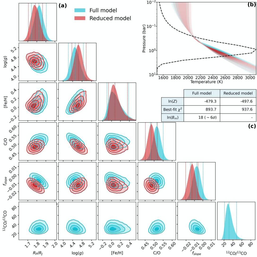
Extended Data Figure 2 | Posteriors of the retrieved parameters and temperature structure for the full (cyan) and reduced (red) models. The vertical dashed lines denote the 5%, 50%, 95% quantiles (90% uncertainties) of the distribution. Panel (b): T-P profile. The shaded regions with decreasing color saturation show 1\sigma , 2\sigma , and 3\sigma temperature uncertainty envelopes respectively. The black dashed line shows the flux average of the emission contribution function. The opaqueness of the temperature uncertainty envelopes has been scaled by this contribution function. Panel (c): fitting statistics of the full and reduced retrieval model, where \ln(Z) and \ln(B_m) represent the logarithm of Bayesian evidence and Bayes factor.
