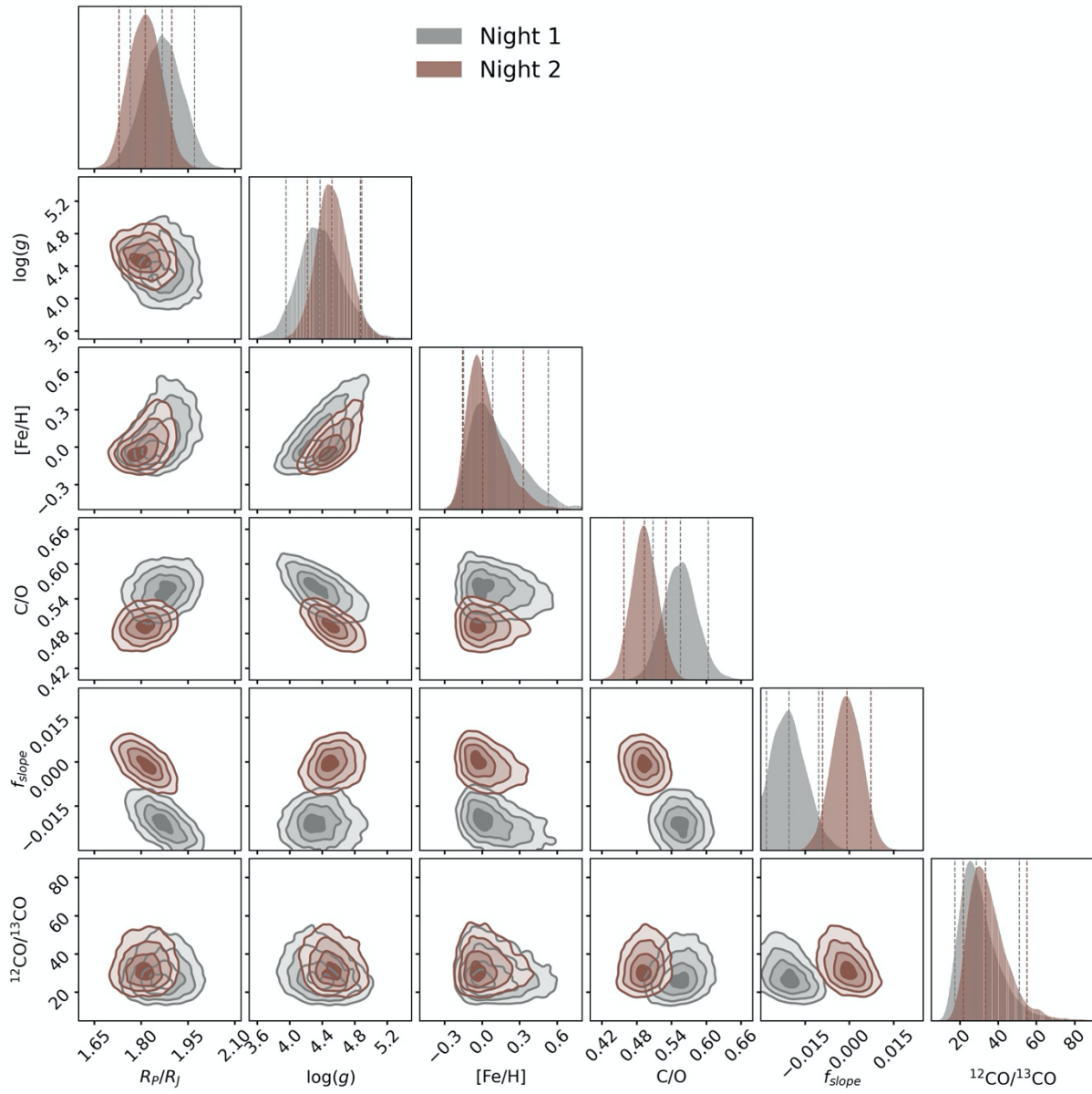
Extended Data Figure 3 | Posteriors of the retrieved parameters for the data of individual nights. Similar as Extended Data Figure 2a.
