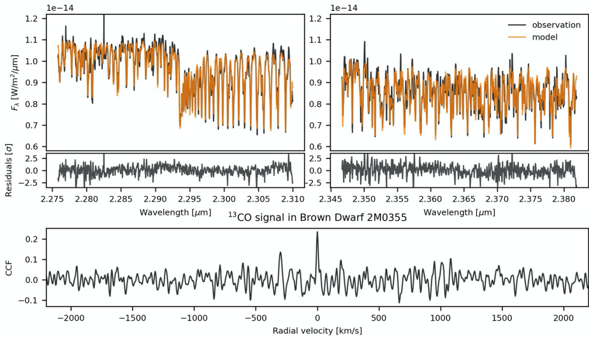
Extended Data Figure 6 | K-band spectrum of the brown dwarf 2M0355 taken by Keck/NIRSPEC and the cross-correlation signal of 13 CO. The black line shows the observed spectrum and the orange line is the best-fit model obtained by retrieval analysis. Bottom panel: Cross-correlation function (CCF) between the 13 CO model and observational residuals. The peak at zero velocity clearly shows the detection of 13 CO.
