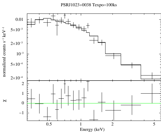
Fig. 20 Simulated SXI spectrum for PSR J1023+0038 in its current sub-luminous LMXB state adopting a 100 ks exposure and an absorbed power law with N_{\text{H}} = 3 \times 10^{20} \text{ cm}^{-2} and \Gamma=1.7 .
