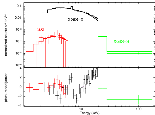
Fig. 9 A simulation of a 25 ks exposure of a MCV with THESEUS. The spectrum was simulated with a multi-temperature plasma emission model (with T_{\max}=45 keV) and a Compton reflection component. An average intrinsic N_H of 5 \times 10^{22} \text{cm}^{-2} is assumed. The count rates are 0.0013 \text{cts s}^{-1} (0.3-6 keV), 0.66 \text{cts s}^{-1} (2-30 keV) and 0.0033 \text{cts s}^{-1} (30-150 keV). The bottom panel shows the residuals obtained when the reflection component is not included in the fit.
