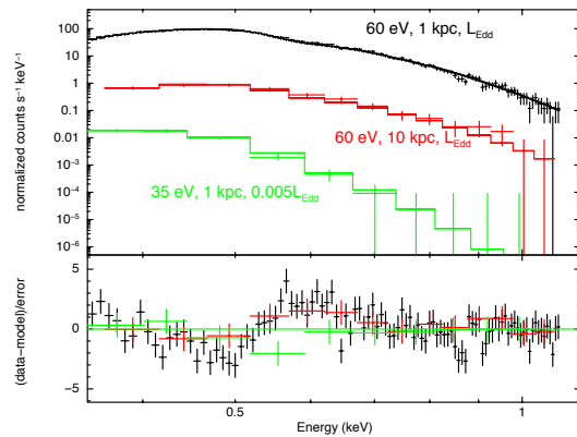
Fig. 12 A simulation of soft X-ray component spectrum of a nova for the SXI instrument using a 60 eV blackbody model with N_H=2 \times 10^{21} cm^{-2} . The black curve assumes a 60 eV blackbody emission with Eddington luminosity at d=1 kpc, giving 21.1 cts s^{-1} in the SXI, whereas the red curve is the same blackbody emission for d=10 kpc simulated for the constant bolometric luminosity phase (2.5 ks, predicted rate 0.22 cts s^{-1} ). The green curve represents a 0.005L_{Edd} of a 35 eV cooling WD after X-ray turn-off with an exposure of 150ks and d=1 kpc.
