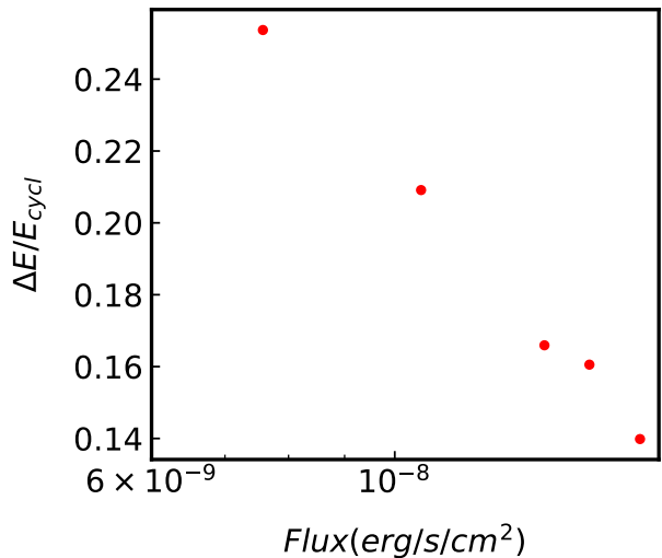
Fig. 15 Relative error (90% c.l.) on the determination of the cyclotron line energy as a function of source observed flux (2-200 keV) for simulated XGIS observations of 70 ks exposure time. We used a spectrum as observed in HMXB Cen X–3 [111], consisting of exponentially cut-off power law with an absorption line at E_c=30.7 keV.
