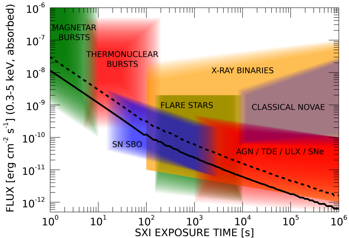
Fig. 1 SXI sensitivity as a function of exposure time for sources with an absorbed power law spectrum with photon index \Gamma=2 and N_H=5\times 10^{20} (solid line) or N_H=10^{22} \text{cm}^{-2} (dashed line). Both curves refer to absorbed source fluxes (0.3-5 keV) with a 95% probability to exceed a detection threshold of 3\sigma (see Appendix for details). Approximate regions of the fluxes and variability time scales expected from different classes of sources are also indicated.
