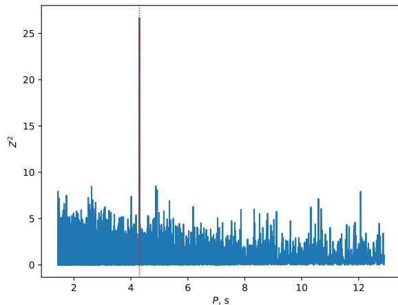
Fig. 14 Simulated periodogram for 10 ks THESEUS/SXI observation (typical daily exposure) for a representative transient X-ray pulsar with bolometric flux of 10^{-9} erg cm ^{-2} s ^{-1} , spin period of 4.3 s and pulsed fraction of 20% (excluding background).
