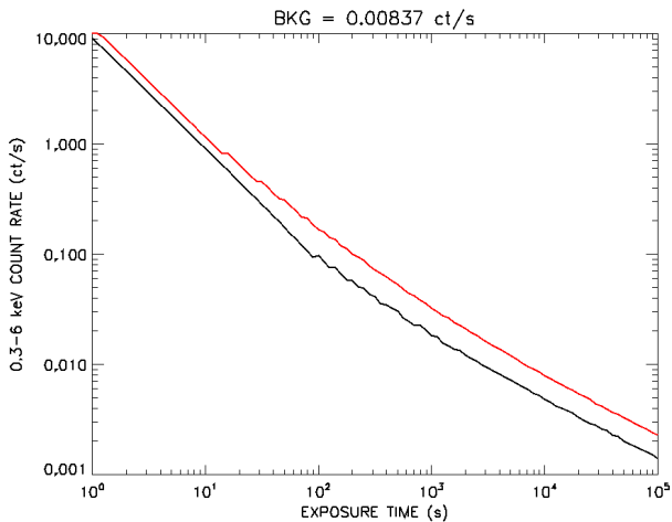
Fig. 36 SXI sensitivity as a function of exposure time. The lower curve (black) gives the count rate corresponding to a 95% probability to exceed a threshold of 3\sigma ( P_1=1.35\times 10^{-3} ), while the upper curve (red) gives the count rate corresponding to a 99% probability to exceed a threshold of 5\sigma ( P_1=3\times 10^{-7} ). The assumed background rate of 8.371\times 10^{-3} cts s^{-1} is appropriate for a source extraction region of 675 arcmin ^2 .
