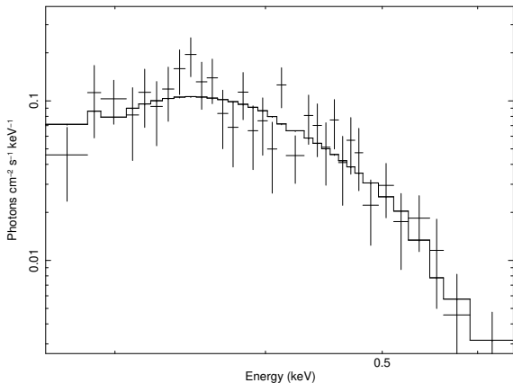
Fig. 31 Simulation of a typical, soft TDE ( kT=50 eV, N_H=1\times 10^{21} \text{cm}^{-2} ) observed for 20 ks with the SXI with a flux of \sim 1\times 10^{-11} \text{erg cm}^{-2} \text{s}^{-1} .
