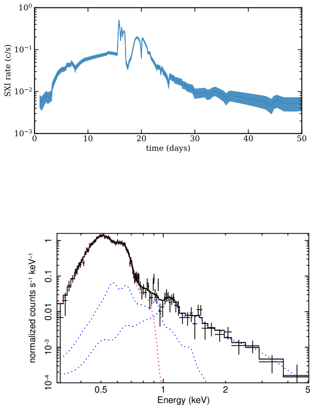
Fig. 13 (a) The top figure shows the predicted SXI count rates that would have been seen from the recurrent nova V3890 Sgr, derived from Swift/XRT observations [95]. The shaded region denotes the 1\text{-}\sigma Poisson error range expected for an exposure time of 2.3 ks, typical for THESEUS visits. (b) The bottom figure shows the predicted SXI spectrum on day 20 of the outburst, as simulated for an exposure of 20 ks (i.e. multiple visits combined) to reveal the hard component. The supersoft source emission dominates the SXI count rate, with the shocked ejecta contributing only 10% of the emission on day 20.
