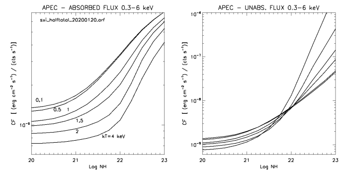
Fig. 38 SXI counts to flux conversion rates for a thermal plasma spectrum (APEC in XSPEC) as a function of absorption. The lines refer to different temperatures. The left figure refers to absorbed fluxes and the right one to fluxes corrected for the absorption.
