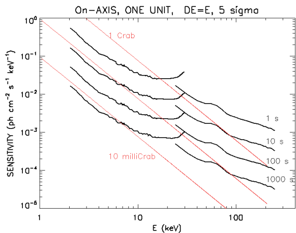
Fig. 3 XGIS imaging sensitivity ( 5\sigma c.l., \Delta E/E=1 ) for different exposure times. The curves refer to a single unit and sources in the fully coded field of view ( \sim 10 \times 10 deg ^2 ). One Crab corresponds to 3 \times 10^{-8} erg cm ^{-2} s ^{-1} in the 2-30 keV range and to 1.6 \times 10^{-8} erg cm ^{-2} s ^{-1} in the 30-150 keV range.
