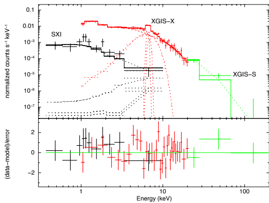
Fig. 10 A 25 ks exposure simulation of a nonmagnetic CV with 2-30 keV flux of 6 \times 10^{-12} erg cm ^{-2} s ^{-1} (see text for details). The count rates in the three detectors are 0.002 cts s ^{-1} (0.3-6 keV), 0.074 cts s ^{-1} (2-30 keV) and 0.0005 cts s ^{-1} (30-150 keV).
