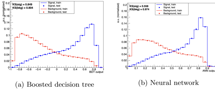
Figure 7.7: Example of the output distribution of the boosted decision tree and neural network for the category with 150 \text{ GeV} < p_T^V < 250 \text{ GeV} , 1 c -tagged jet and 3 jets or more in the event.
