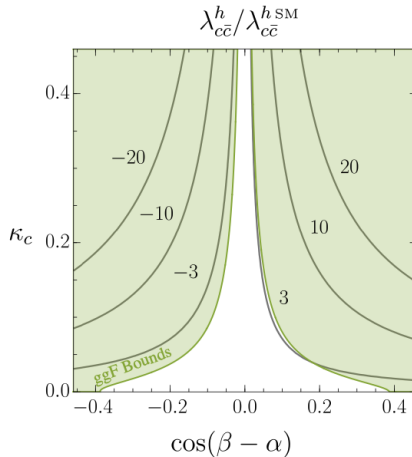
Figure 2.5: Enhance coupling of the Higgs boson of the SM with charm quarks \lambda_{c\bar{c}}^h / \lambda_{c\bar{c}}^{h_{SM}} as a function of the Yukawa couplings \kappa_c of the second Higgs field \phi' and the alignment parameter \cos(\beta - \alpha) . The notation of the paper [15] is used and the \kappa_c parameter is not the same as the \kappa_i in Fig. 2.4 and generally the \kappa framework. The green bands are obtained from the experimental measurement of the SM Higgs boson measured in the gluon-gluon fusion (ggF) production mode and a decay to two photons H \rightarrow \gamma\gamma .
