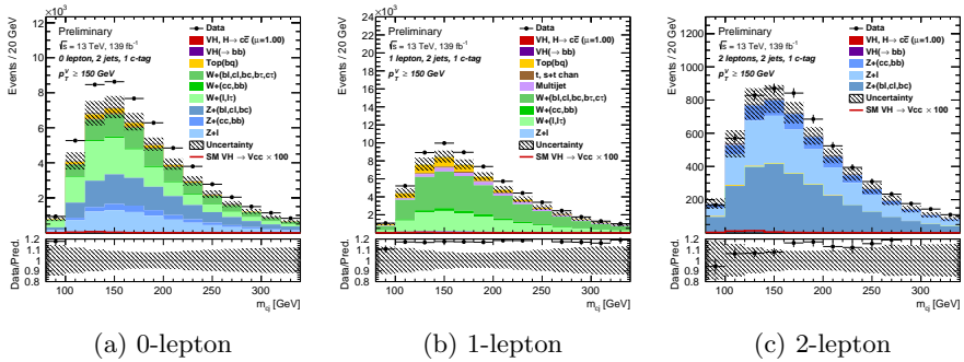
Figure 5.24: Example of the high \Delta R CR for the category with 2 jets and p_T^V > 150 \text{ GeV} .
