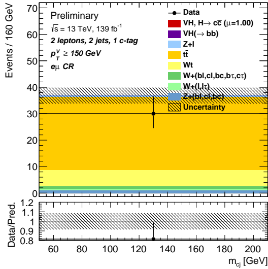
Figure 5.27: Example of the top- e\mu control region for the 2-lepton channel in the category with 1 c -tag and 2 jets and p_T^V > 150 \text{ GeV} .
