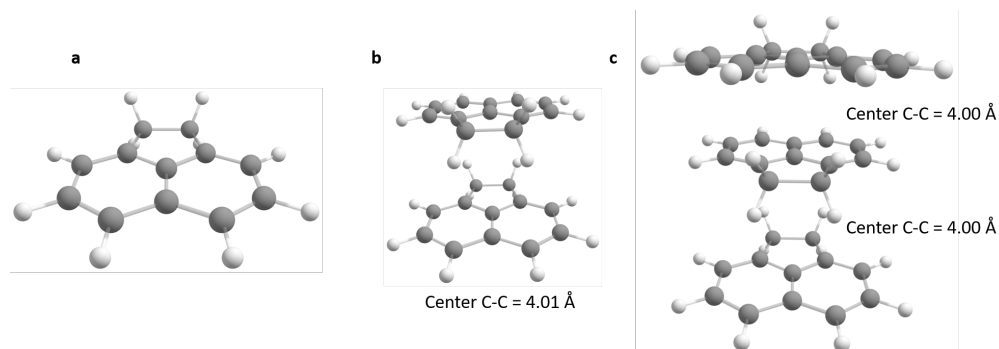
Figure 6.4: The calculated structures of Ace_n ( n = 1-3 ) complexes at the PBEh-3c level of theory.
