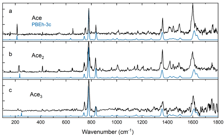
Figure 6.3: Mid- to far-infrared gas phase action spectra of jet cooled Ace_n ( n = 1-3 ) complexes in black. Displayed in blue are the corresponding calculated spectra at the PBEh-3c level of theory (uncorrected, but scaled with 0.95).
