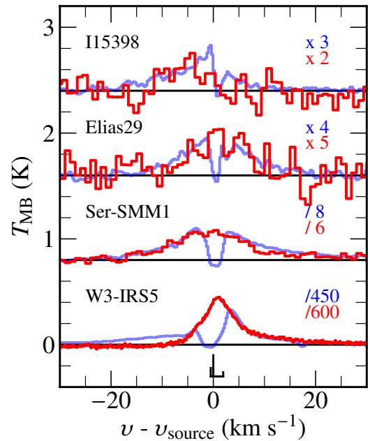
Fig. 15. Comparison of HIFI spectra of the H 2 O 1_{10}\text{--}1_{01} 557 GHz line (blue) and the OH 1834 GHz triplet (red) toward a number of low and high-mass regions. The splitting of the three OH lines in the triplet and their relative strength are indicated at the bottom of the figure. Data from Kristensen & Wampfler (priv. comm.).
