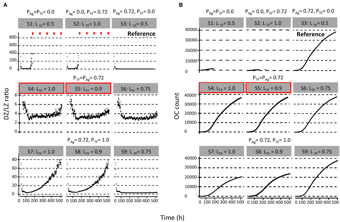
FIGURE 3 | Results from first set of simulations (Table 2). (A) DZ-to-LZ ratio and (B) accumulated OCs during the GC reaction. The probability of asymmetric division (P) is indicated above the gray box, and simulation number and polarity levels (L) are shown in the gray box. Red dots indicate DZ-to-LZ ratio values of infinity. First row of plots corresponds to (left column) symmetric division of Ag and TFs, (middle column) symmetric division of Ag and asymmetric division of TFs, and (right column) symmetric division of TFs and asymmetric division of Ag. Second row of plots corresponds to asymmetric TF division only if mode of Ag division is asymmetric. Red boxes indicate parameters that are closer to biological results. Third row of plots corresponds to always asymmetric TF division regardless of mode of Ag division.
