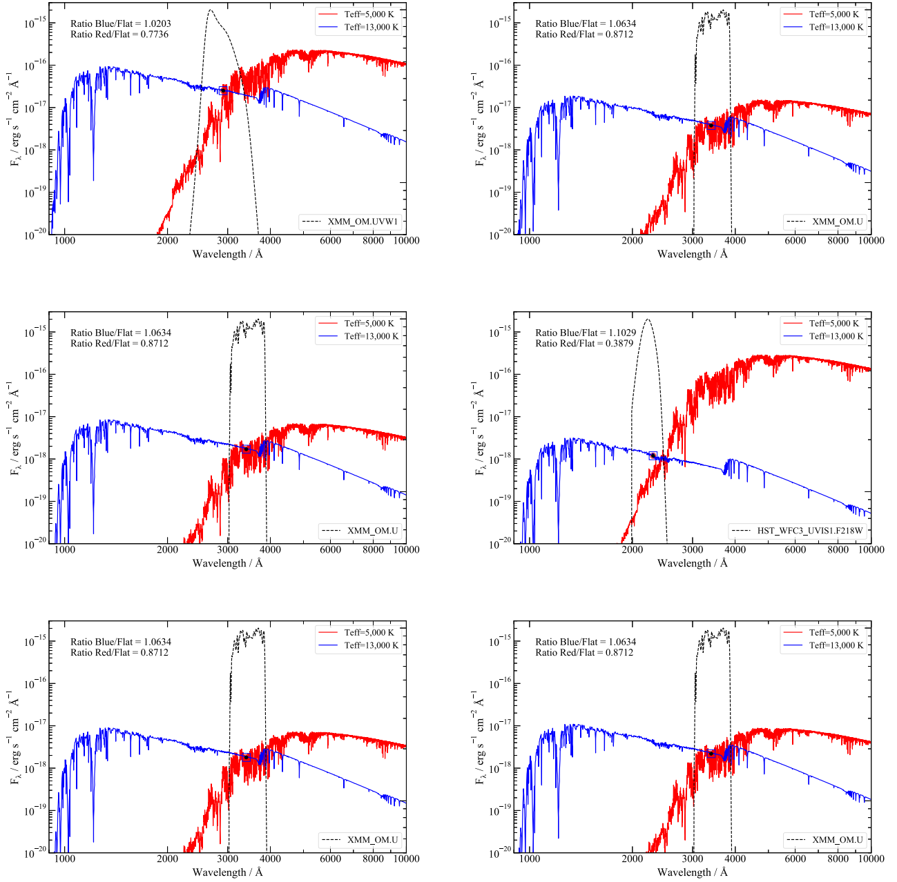
Figure A1. Estimates of the effect of the unknown UV spectral shape on the inferred UV luminosity. For each observation, we show the measured UV flux (upper limit) as the black data point, while the blue and red curves represent blackbody spectra with temperatures of 13 000 and 5000 K, respectively. The black dashed curves show the different filter transmissions. Printed in the top left are the ratios of the integrated fluxes for these models compared to a flat distribution over the filter passband. These plots show that the unknown spectral shape has a relatively minor impact on the calculated U -band luminosity (of order 10 per cent), but has an increasingly large impact for bluer filters.
