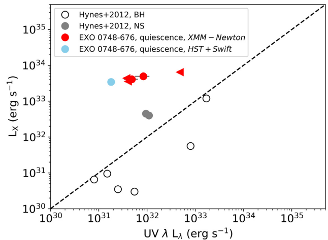
Figure 3. The observed X-ray versus UV luminosity of EXO 0748–676 during six quiescent epochs is shown. Five epochs were obtained using XMM-Newton (shown in red). One epoch was observed using HST and the Swift , and is shown in blue. We note that these data points do not take into account the unknown UV spectral shape (see Section A1). We compare EXO 0748–676 to eight other quiescent LMXBs studied in Hynes & Robinson (2012). The six systems hosting BHs are shown by open black circles and represent GRO J0422+32 (V518 Per), MM Vel, XTE J118–40, A0620–00, GU Mus, and V404 Cyg (listed in ascending order of the UV luminosity). The two NS systems are shown by filled grey circles and correspond to Aql X-1 and Cen X-4. All upper limits are marked by triangles facing the relevant direction.
