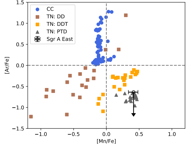
Figure 6. [\text{Ar}/\text{Fe}]-[\text{Mn}/\text{Fe}] diagram for four groups of explosion mechanisms plotted in Figures 4 and 5. The observed ratios in Sgr A East are overplotted for comparison. The dashed lines denote the solar values for [\text{Mn}/\text{Fe}] and [\text{Ar}/\text{Fe}] .
