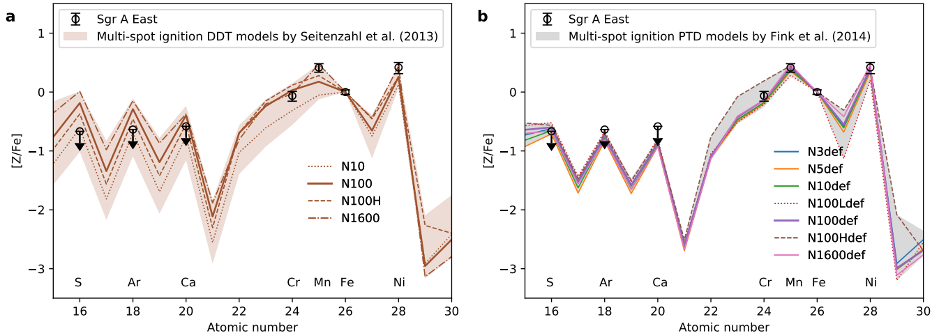
Figure 5. Comparison between the observed logarithmic abundance ratios (relative to Fe) and offcentered mutispot ignition DDT (a) and PTD models (b). All available models have been considered in the shaded region, but a few exemplified models are shown with lines. N10(def) and N100(def) mean 10 and 100 ignition bubbles, respectively. In panel (b), the initial central density of the WD is 2.9 \times 10^9 \text{ g cm}^{-3} for the N3–1600def models, 10^9 \text{ g cm}^{-3} for the N100Ldef model and 5.5 \times 10^9 \text{ g cm}^{-3} for the N100Hdef model.
