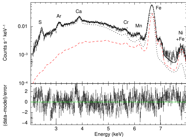
Figure 2. Chandra ACIS-S spectrum in 2–8 keV fitted with an absorbed two-temperature model tbabs * (vvapec + vvapec) . The dotted line and the red dashed line denote the cool and hot components, respectively. Spectral fit results are shown in Table 1.
