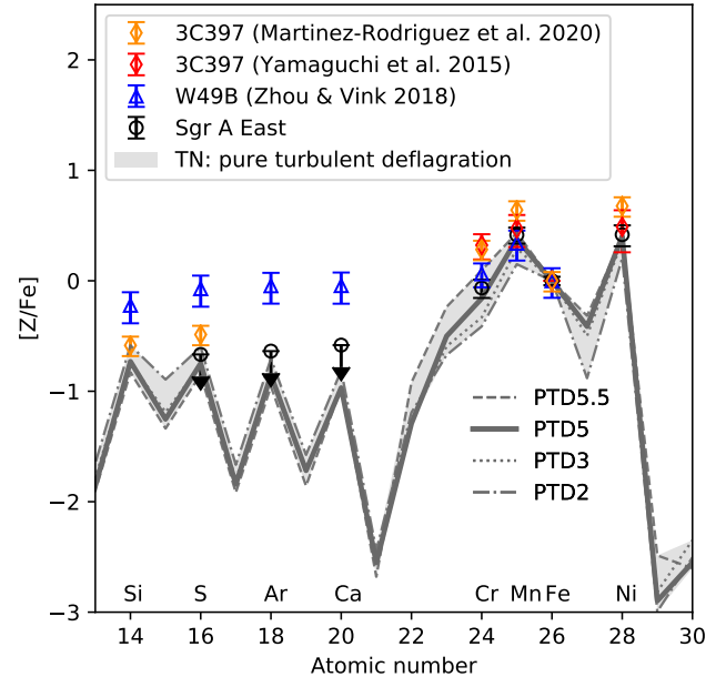
Figure 7. Comparison between the observed logarithmic abundance ratios (relative to Fe) for 3C 397, W49B, and Sgr A East and the PTD models by Leung & Nomoto (2020a). We adopted a 20% systematic error for the ratios from Martínez-Rodríguez et al. (2020), which have very small statistical errors.
