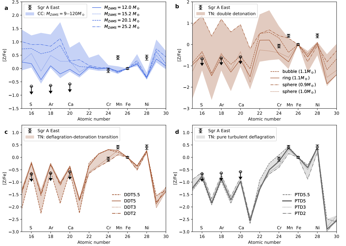
Figure 4. A comparison between the observed logarithmic abundance ratios (relative to Fe) and core-collapse (CC) and thermonuclear (TN) nucleosynthesis models. The error bars give 90% uncertainties. (a) core-collapse SN models for stars with zero-age-main-sequence masses from 9 to 120 M_{\odot} (Sukhbold et al. 2016). (b) double detonation Type Ia models for sub-Chandrasekhar-mass WDs (0.9–1.2 M_{\odot} ) with three initial He detonation configurations (Leung & Nomoto 2020b). Three benchmark models and a low-mass WD model (0.9 M_{\odot} WD) are labeled with lines. (c) deflagration-detonation transition (DDT) Type Ia SN models for C+O WDs with central densities of 2 \times 10^9 (DDT2), 3 \times 10^9 (DDT3), 5 \times 10^9 \text{g cm}^{-3} (DDT5), and 5.5 \times 10^9 \text{g cm}^{-3} (DDT5.5), respectively (Leung & Nomoto 2018). (d) pure turbulent deflagration (PTD) Type Iax SN models (Leung & Nomoto 2020a) for WDs with central densities in the range of 2.0 – 5.5 \times 10^9 \text{g cm}^{-3} (PTD2–5.5). The thick solid line shows the best-fit Type Iax model with a central density of 5 \times 10^9 \text{g cm}^{-3} .
