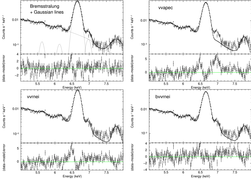
Figure 3. Chandra ACIS-S spectrum in 5–8 keV fitted with single thermal component models. Top left: the spectrum in 5–8 keV fitted using absorbed bremsstrahlung+Gaussian lines (see Table 2 for the fitting results); top right: vvapec ; bottom left: recombining plasma model vvrnei ; and bottom right: recombining plasma model bvvrnei with a velocity broadening.
