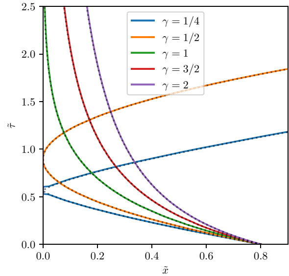
FIG. 3. Position as a function of time of a Gaussian wave packet in the lattice model for five values of \gamma , with x_0 = 800, p_0 = -\pi/2, w = 50, and N = 1001 . The solid lines represent numerical calculations, while the dashed lines represent Eq. (7). For \gamma < 1 , the wave packet bounces on the origin of the lattice, while for \gamma \geq 1 , it reaches the end of the lattice asymptotically.
