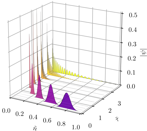
FIG. 2. Time evolution of a Gaussian wave packet in the lattice model, with \gamma = 1, n_0 = 800, p_0 = -\pi/2, w = 50, and N = 1001 . The wave packet slows down and localizes at the origin of the lattice, where it disintegrates.
