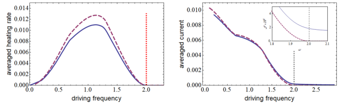
FIG. 5. Averaged heating rate \overline{\mathcal{W}} (left) and current \overline{\mathcal{J}} (right) for a QPC with J_t = 0.3 \sin \omega t , U_t^L = -U_t^R = 0.3 \cos \omega t calculated numerically (solid lines; the system size and initial state are the same as in Fig. 4) and perturbatively [dashed lines; see Eqs. (19) and (20), respectively]. Both the average heating rate and current vanish for \omega \geq 2 in the leading order. However, the actual current remains finite due to the higher-order corrections, as illustrated in the inset in the right panel.
