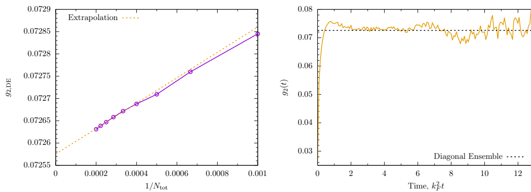
Figure 15: The scaling with N_{\text{tot}} of the diagonal ensemble result (left panel) for c_i = 20 \rightarrow c_f = 10 quench with N = 10 particles. The dotted line shows a linear extrapolation to N_{\text{tot}} = \infty . A comparison of the N_{\text{tot}} = 3500 data of Fig. 13 with the extrapolated diagonal ensemble result for the long time limit (right panel).
