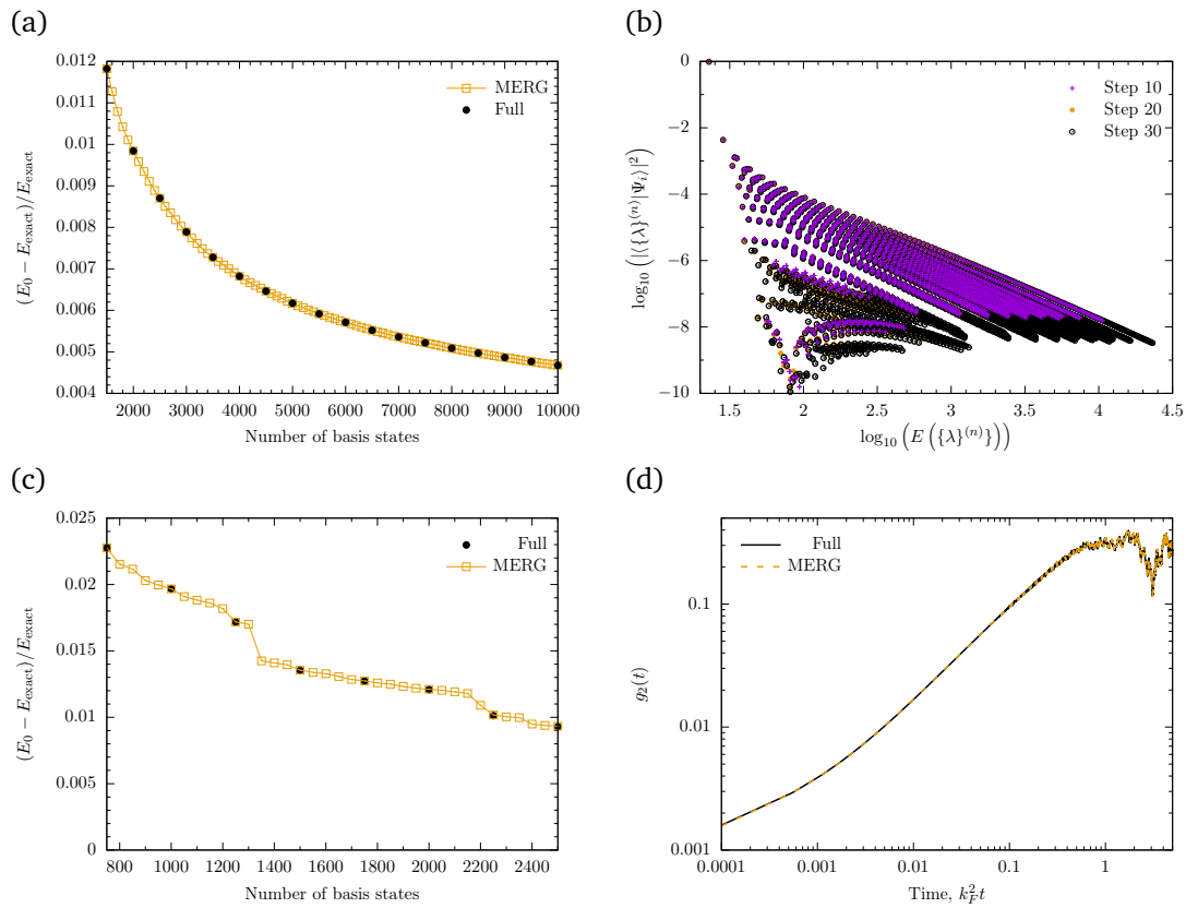
Figure 18: Top row: Matrix element renormalization group (MERG) and numerical renormalization group (NRG) for the c_i = 20 \rightarrow c_f = 10 quench for N = 10 particles, computed within the high overlap states truncation scheme. (a) The convergence of the initial state energy as a function of number of basis states; (b) the convergence of the overlaps at different steps of the MERG procedure (cf. Fig. 9). Bottom row: MERG and full diagonalization results for the N = 4 particle quench c_i = 100 \rightarrow c_f = 3.7660 : (c) the convergence of the energy of the initial state with the number of basis states; (d) the time evolution of g_2(t) with 2500 basis states.
