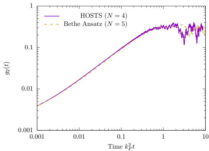
Figure 14: The time evolution of the local observable g_2(t) following the c_i = 100 \rightarrow c_f = 3.7660 in the Lieb-Liniger model starting from the ground state at c_i with unit density. Exact data (dashed line) computed via the coordinate Bethe ansatz with N = 5 particles (from Ref. [45]) is compared to high overlap states truncation scheme (HOSTS) computations with N = 4 particles. HOSTS results for higher numbers of particles are discussed in Sec. 5.
