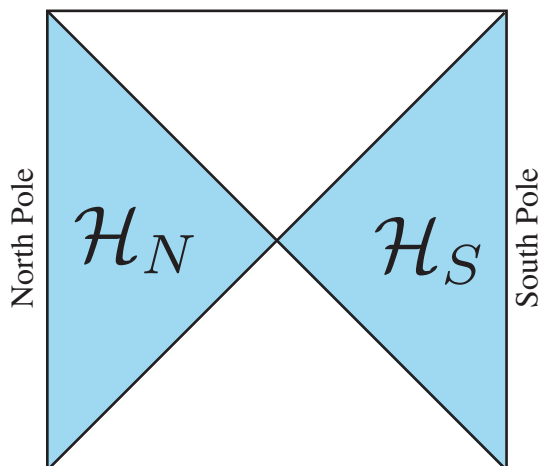
Figure 1. Two antipodal static patch regions (shaded blue). The thermofield double state with Hilbert space \mathcal{H}_{\text{TFD}} = \mathcal{H}_N \otimes \mathcal{H}_S is constructed by maximally entangling the two static patches.
