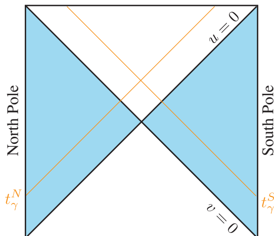
Figure 2. De Sitter Penrose diagram and global lightcone coordinates. The two static patches are shaded blue.
