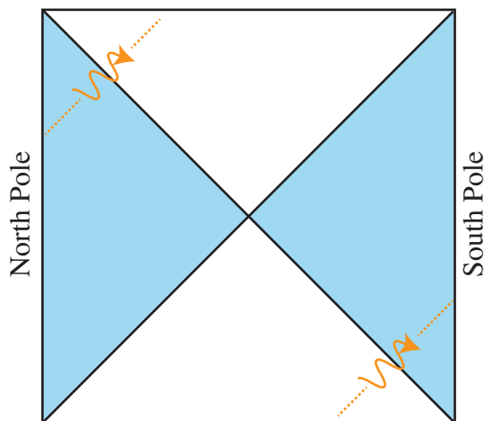
Figure 5. In the thermofield double state, for each mode there is a maximally entangled mirror mode across the horizon.
