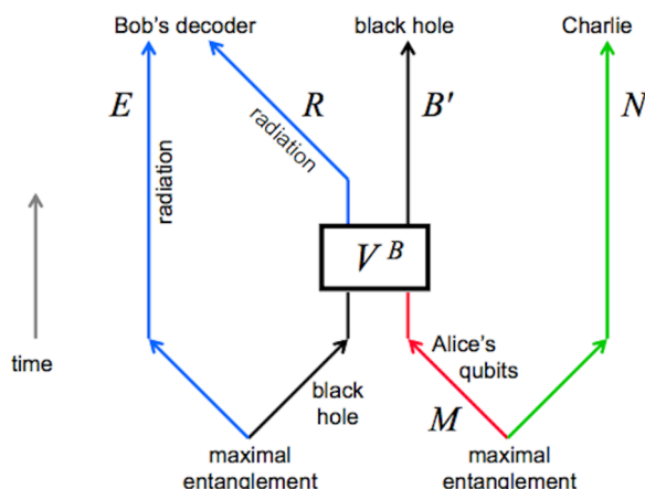
Figure 4. Quantum circuit corresponding to the Hayden-Preskill protocol. Figure from [21].
