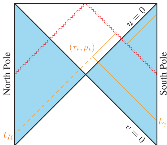
Figure 7. A message leaving the South Pole is reflected and after crossing the shockwave returns to the pole.
