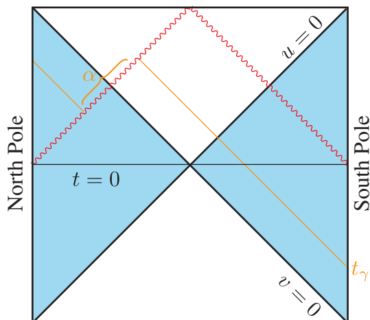
Figure 3. A pair of shockwaves in de Sitter space and a shifted lightray.
