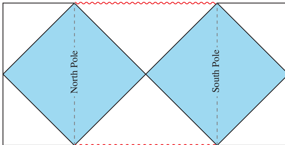
Figure 6. The Schwarzschild-de Sitter causal diagram showing the shared exterior, as well as a shared black hole interior, between two (previously) antipodal observers. As the black hole is removed the interior geometry of the black hole is replaced with a de Sitter exterior geometry.
