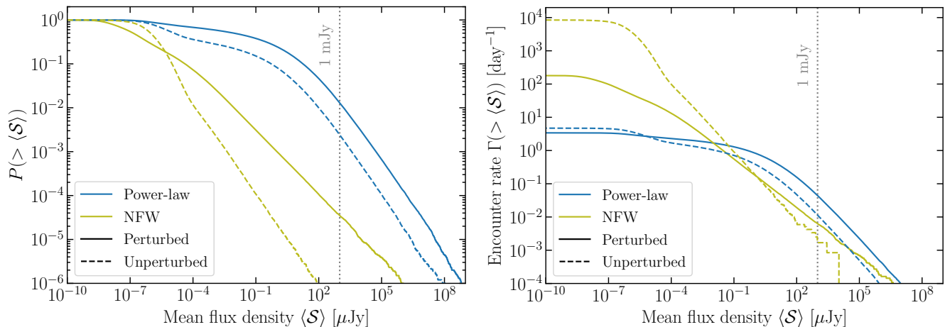
FIG. S2. Left : The cumulative probability of AMC-NS encounters as a function of the mean flux \langle S \rangle of the resulting radio signal. Right : Cumulative rate of encounters above a given mean flux \langle S \rangle .
