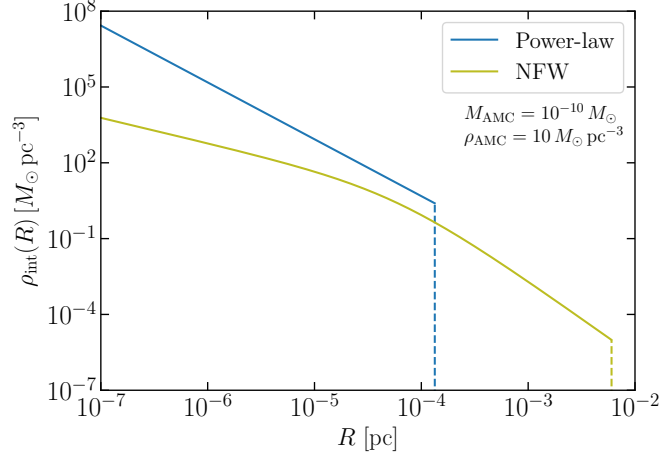
FIG. S1. Models for the internal density profile's of AMCs which we consider in this paper: Power-law, Eq. (S7), and NFW, Eq. (S9). Vertical dashed lines show the truncation radii R_{\text{AMC}} . We fix the characteristic mass and density to M_{\text{AMC}} = 10^{-10} M_{\odot} and \rho_{\text{AMC}} = 10 M_{\odot} \text{pc}^{-3} respectively.
