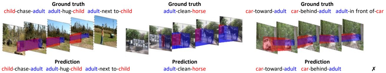
Figure 6: Success and failure cases on VidOR. For the left example, we detect all the ground truth relation instances and successfully predict the long-range relation chase . The middle case needs temporal context information to detect an adult cleaning a horse. Our method’s detection proves its ability to detect long-range relations. In the right example, our approach detects behind and toward relations. But since the object detector wrongly recognizes car as truck , the final triplet predictions are wrong even though the relation predicates are correct. Incorrect object categories also lead to imprecise semantic features, which may contribute to the missing of a relation prediction. We provide more qualitative results and example videos with success and failure in the supplemental material.
