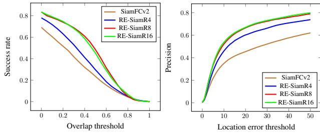
Figure 7: Performance curves for Rot-OTB100 dataset obtained using SiamFCv2 and RE-SiamNet with different choices of equivariant rotation groups. All networks chosen here used 233K optimization parameters.
