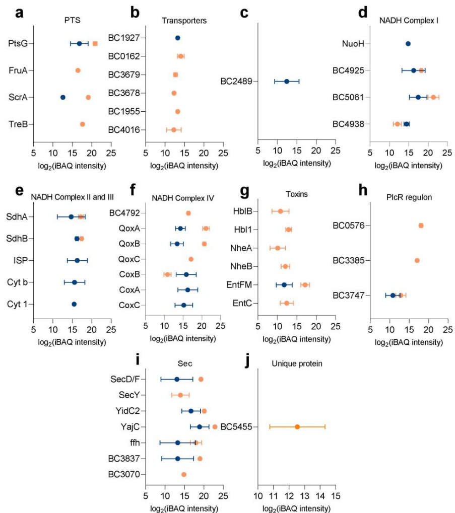
Figure 5. Abundances of proteins with vital functions in the cell or spore membrane. The iBAQ values of proteins from spore inner membrane (blue) and from the vegetative cell membrane (orange) associated with PTS (a), transporters (b), acetyl-coenzyme A synthetase (c), NADH complex I (d), NADH complex II and III (e), NADH complex IV (f), toxins (g), PlcR regulon (h), Sec system (i) and a unique protein (j) are shown, see text for details.
