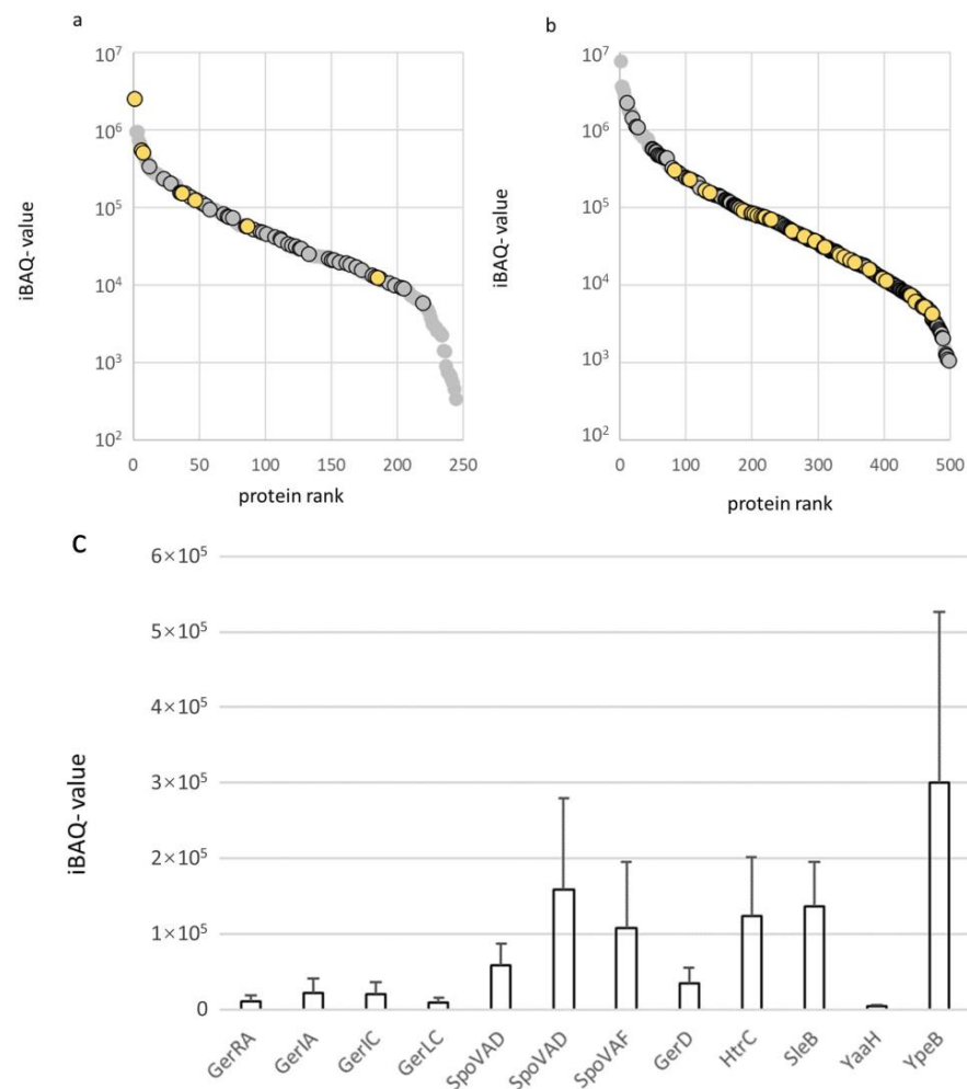
Figure 4. Abundance of membrane annotated proteins in the cell and spore membrane fractions. Membrane annotated proteins are shown ranked according to iBAQ values for spore inner membrane (a) and cell membrane preparations (b). Circles with a solid border mark protein exclusively identified in spores and cells, yellow circles mark uncharacterized proteins. (c) Proteins related to germination of bacillus spores, mean iBAQ values of 3 replicates are shown, error bars denote the standard error of the mean.
